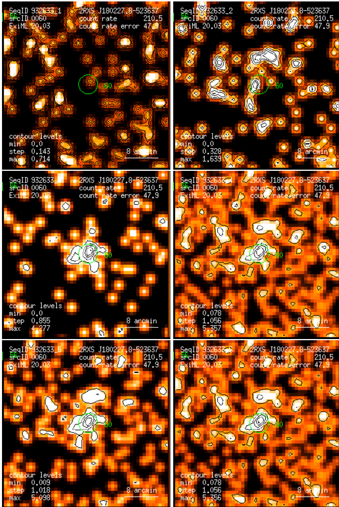
Figure 60: RASS 932633: detection 0060: band rate images, Gaussian filter: (1) PSPC channels 11 – 41, (2) 52 – 90, (3) 91 – 201, (4) 11 – 235, (5) 52 – 201, (6) 11 – 201. Broad band rates in counts/ks. Band rate contour levels in counts/ks/arcmin 2 .
