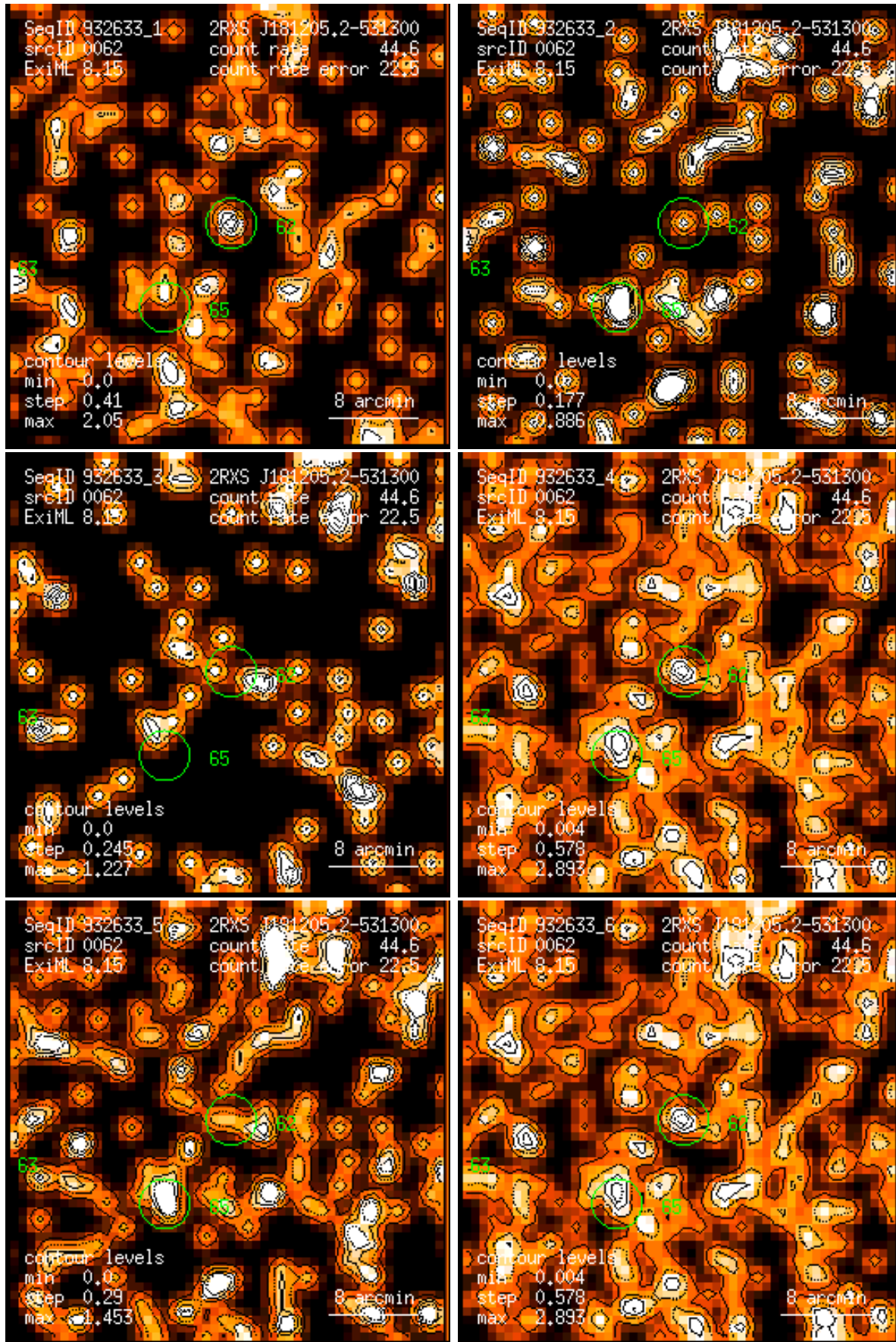
Figure 62: RASS 932633: detection 0062: band rate images, Gaussian filter: (1) PSPC channels 11 – 41, (2) 52 – 90, (3) 91 – 201, (4) 11 – 235, (5) 52 – 201, (6) 11 – 201. Broad band rates in counts/ks. Band rate contour levels in counts/ks/arcmin 2 .
