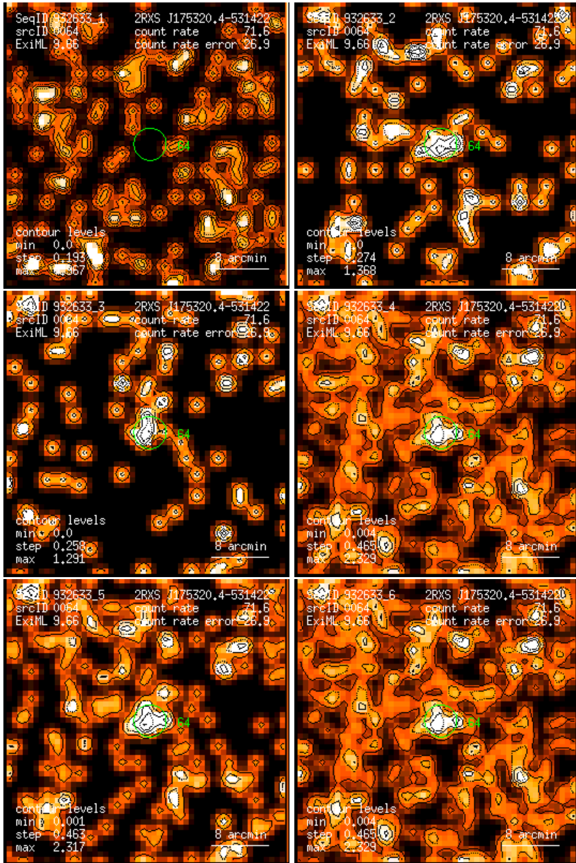
Figure 64: RASS 932633: detection 0064: band rate images, Gaussian filter: (1) PSPC channels 11 – 41, (2) 52 – 90, (3) 91 – 201, (4) 11 – 235, (5) 52 – 201, (6) 11 – 201. Broad band rates in counts/ks. Band rate contour levels in counts/ks/arcmin 2 .
