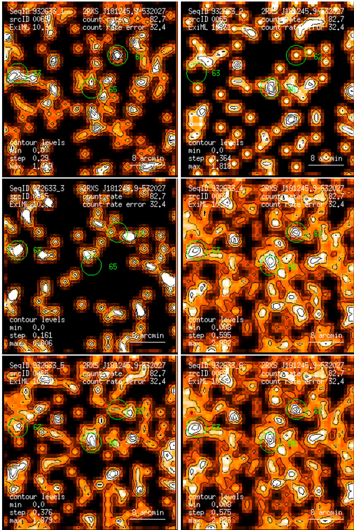
Figure 65: RASS 932633: detection 0065: band rate images, Gaussian filter: (1) PSPC channels 11 – 41, (2) 52 – 90, (3) 91 – 201, (4) 11 – 235, (5) 52 – 201, (6) 11 – 201. Broad band rates in counts/ks. Band rate contour levels in counts/ks/arcmin 2 .
