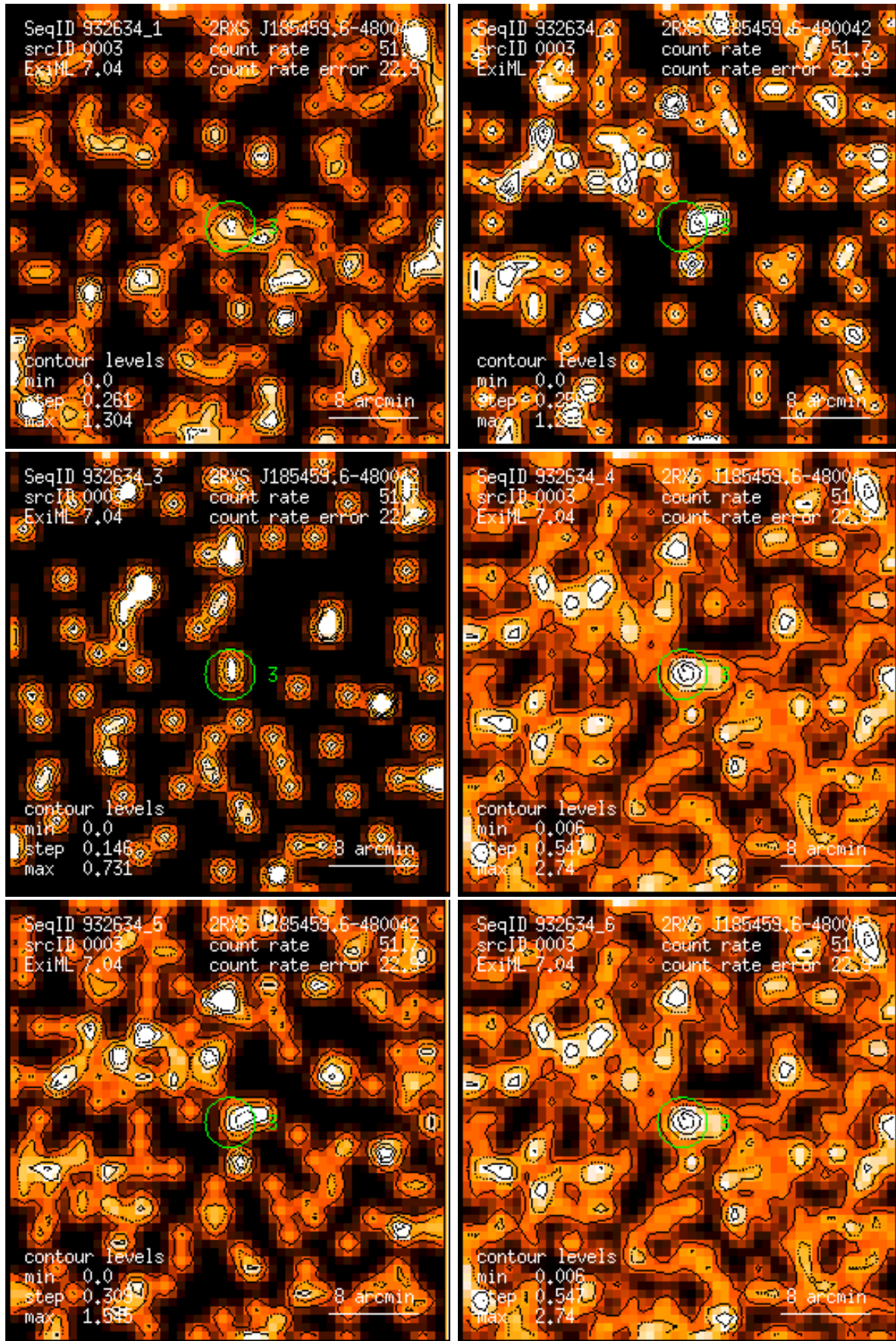
Figure 3: RASS 932634: detection 0003: band rate images, Gaussian filter: (1) PSPC channels 11 – 41, (2) 52 – 90, (3) 91 – 201, (4) 11 – 235, (5) 52 – 201, (6) 11 – 201. Broad band rates in counts/ks. Band rate contour levels in counts/ks/arcmin 2 .
