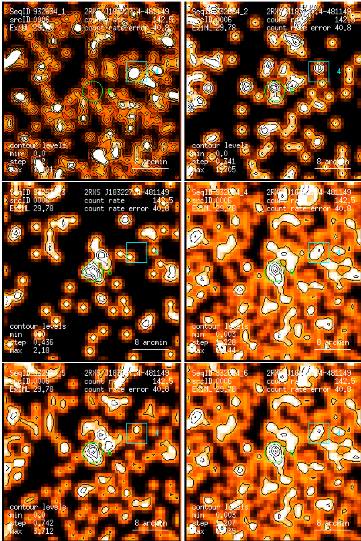
Figure 6: RASS 932634: detection 0006: band rate images, Gaussian filter: (1) PSPC channels 11 – 41, (2) 52 – 90, (3) 91 – 201, (4) 11 – 235, (5) 52 – 201, (6) 11 – 201. Broad band rates in counts/ks. Band rate contour levels in counts/ks/arcmin 2 .
