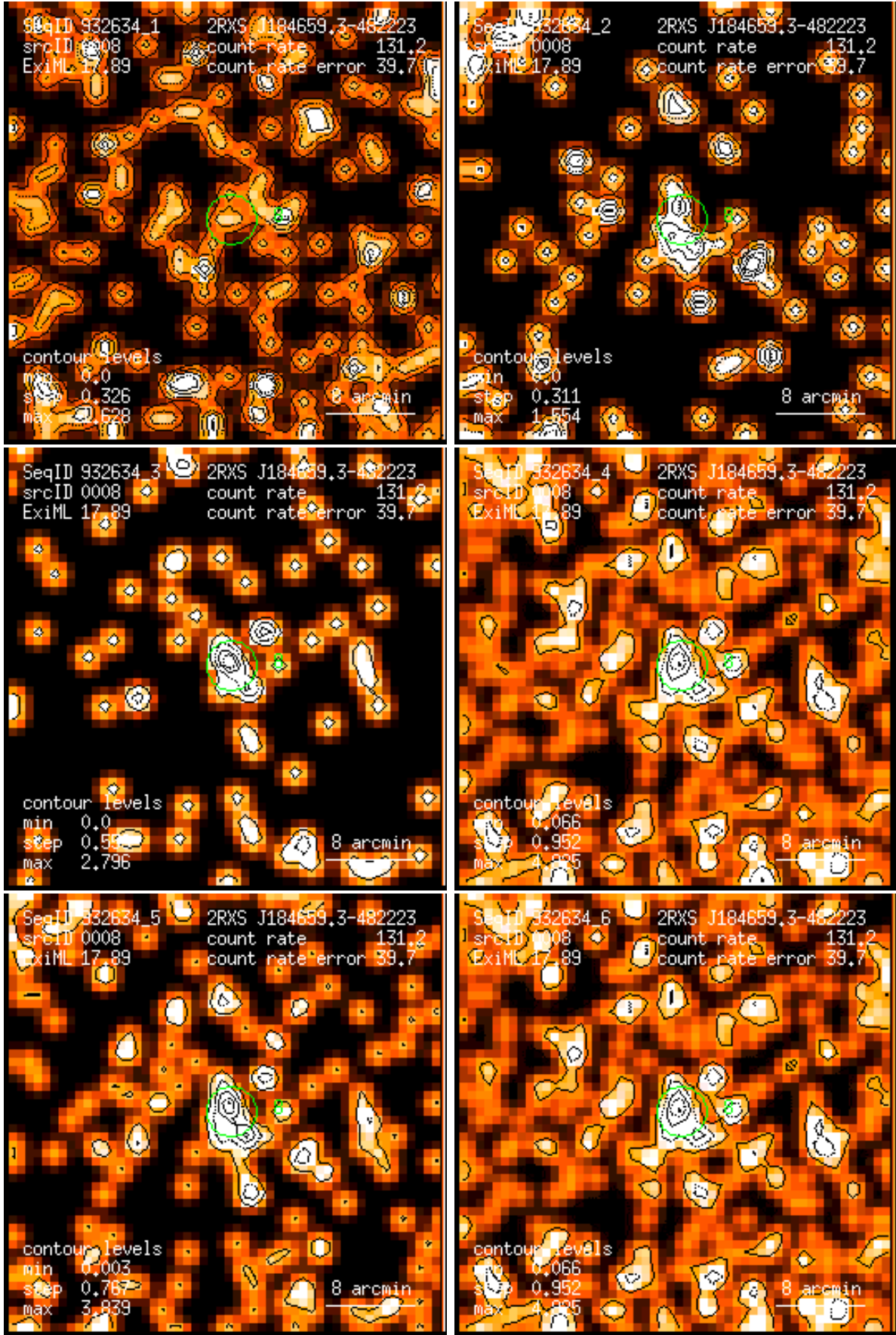
Figure 8: RASS 932634: detection 0008: band rate images, Gaussian filter: (1) PSPC channels 11 – 41, (2) 52 – 90, (3) 91 – 201, (4) 11 – 235, (5) 52 – 201, (6) 11 – 201. Broad band rates in counts/ks. Band rate contour levels in counts/ks/arcmin 2 .
