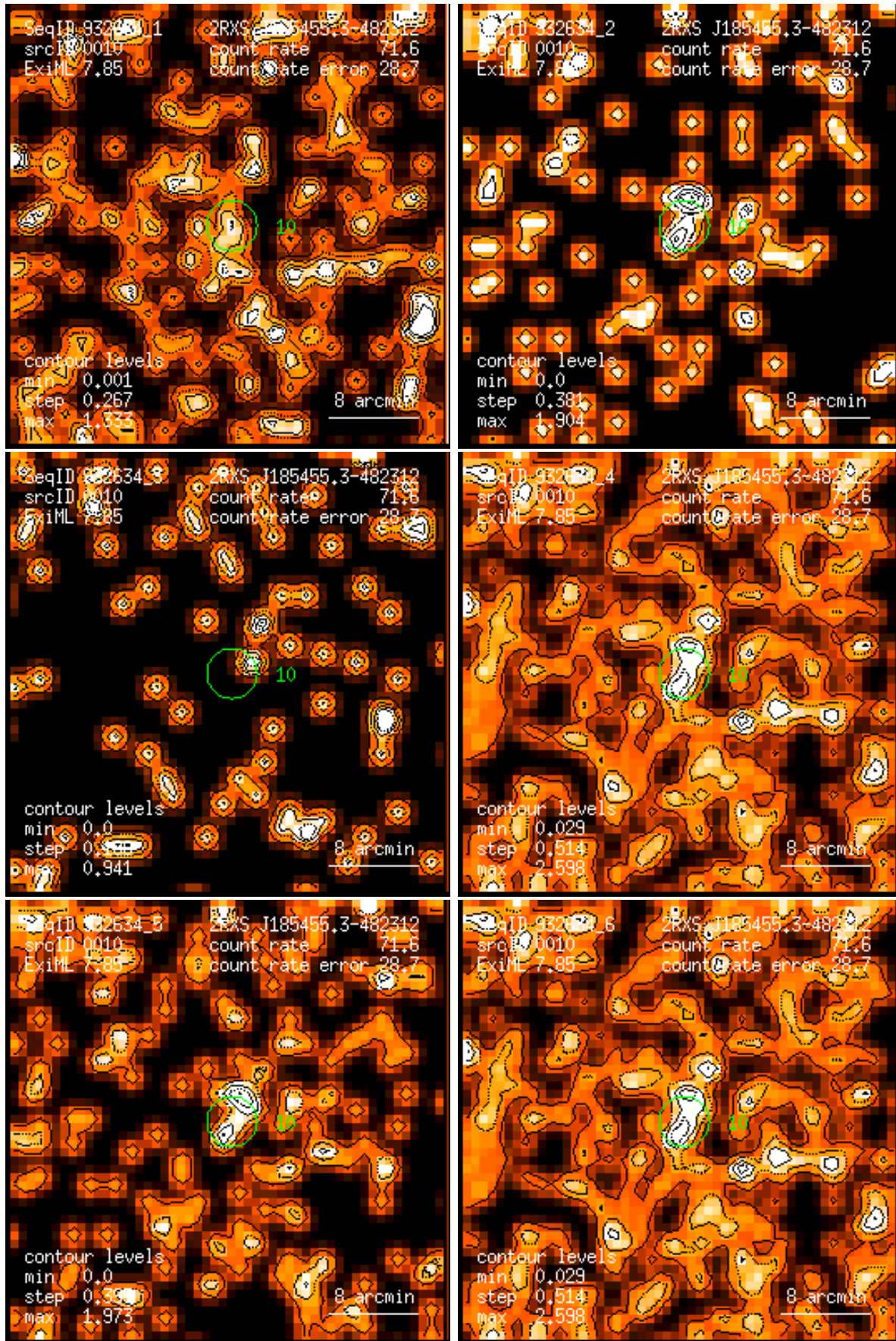
Figure 10: RASS 932634: detection 0010: band rate images, Gaussian filter: (1) PSPC channels 11 – 41, (2) 52 – 90, (3) 91 – 201, (4) 11 – 235, (5) 52 – 201, (6) 11 – 201. Broad band rates in counts/ks. Band rate contour levels in counts/ks/arcmin 2 .
