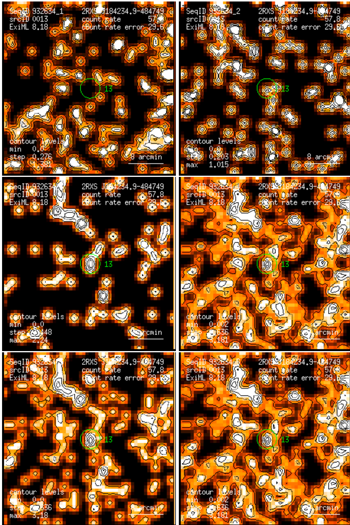
Figure 13: RASS 932634: detection 0013: band rate images, Gaussian filter: (1) PSPC channels 11 – 41, (2) 52 – 90, (3) 91 – 201, (4) 11 – 235, (5) 52 – 201, (6) 11 – 201. Broad band rates in counts/ks. Band rate contour levels in counts/ks/arcmin 2 .
