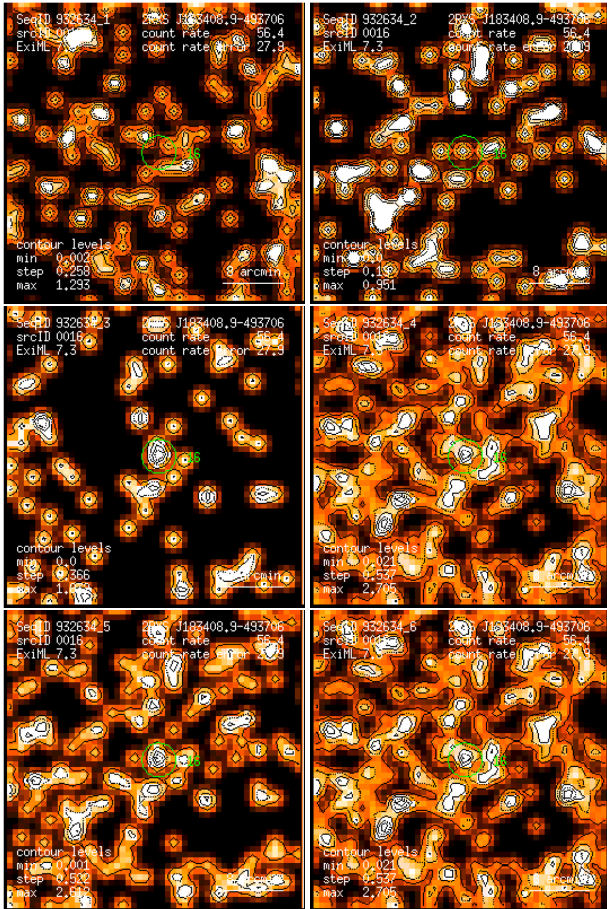
Figure 16: RASS 932634: detection 0016: band rate images, Gaussian filter: (1) PSPC channels 11 – 41, (2) 52 – 90, (3) 91 – 201, (4) 11 – 235, (5) 52 – 201, (6) 11 – 201. Broad band rates in counts/ks. Band rate contour levels in counts/ks/arcmin 2 .
