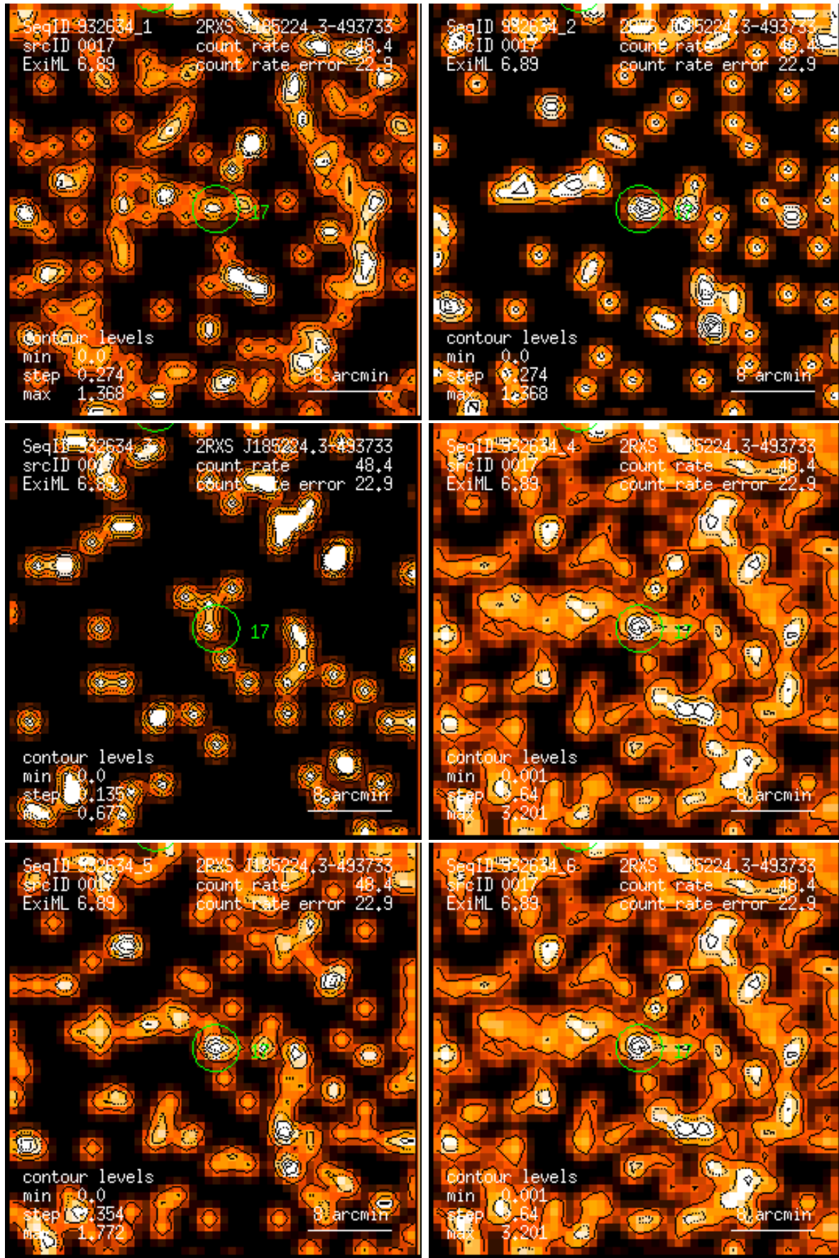
Figure 17: RASS 932634: detection 0017: band rate images, Gaussian filter: (1) PSPC channels 11 – 41, (2) 52 – 90, (3) 91 – 201, (4) 11 – 235, (5) 52 – 201, (6) 11 – 201. Broad band rates in counts/ks. Band rate contour levels in counts/ks/arcmin 2 .
