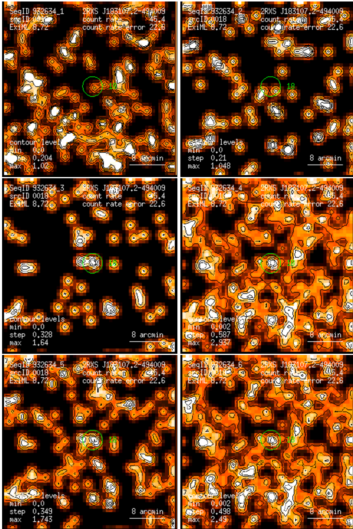
Figure 18: RASS 932634: detection 0018: band rate images, Gaussian filter: (1) PSPC channels 11 – 41, (2) 52 – 90, (3) 91 – 201, (4) 11 – 235, (5) 52 – 201, (6) 11 – 201. Broad band rates in counts/ks. Band rate contour levels in counts/ks/arcmin 2 .
