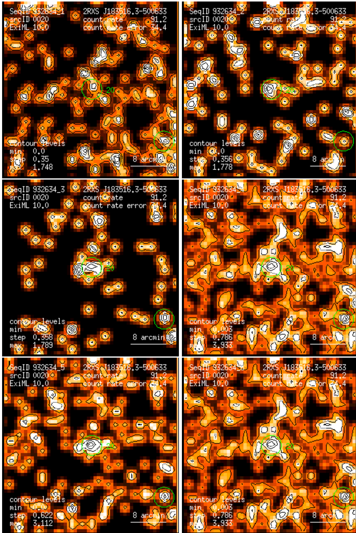
Figure 20: RASS 932634: detection 0020: band rate images, Gaussian filter: (1) PSPC channels 11 – 41, (2) 52 – 90, (3) 91 – 201, (4) 11 – 235, (5) 52 – 201, (6) 11 – 201. Broad band rates in counts/ks. Band rate contour levels in counts/ks/arcmin 2 .
