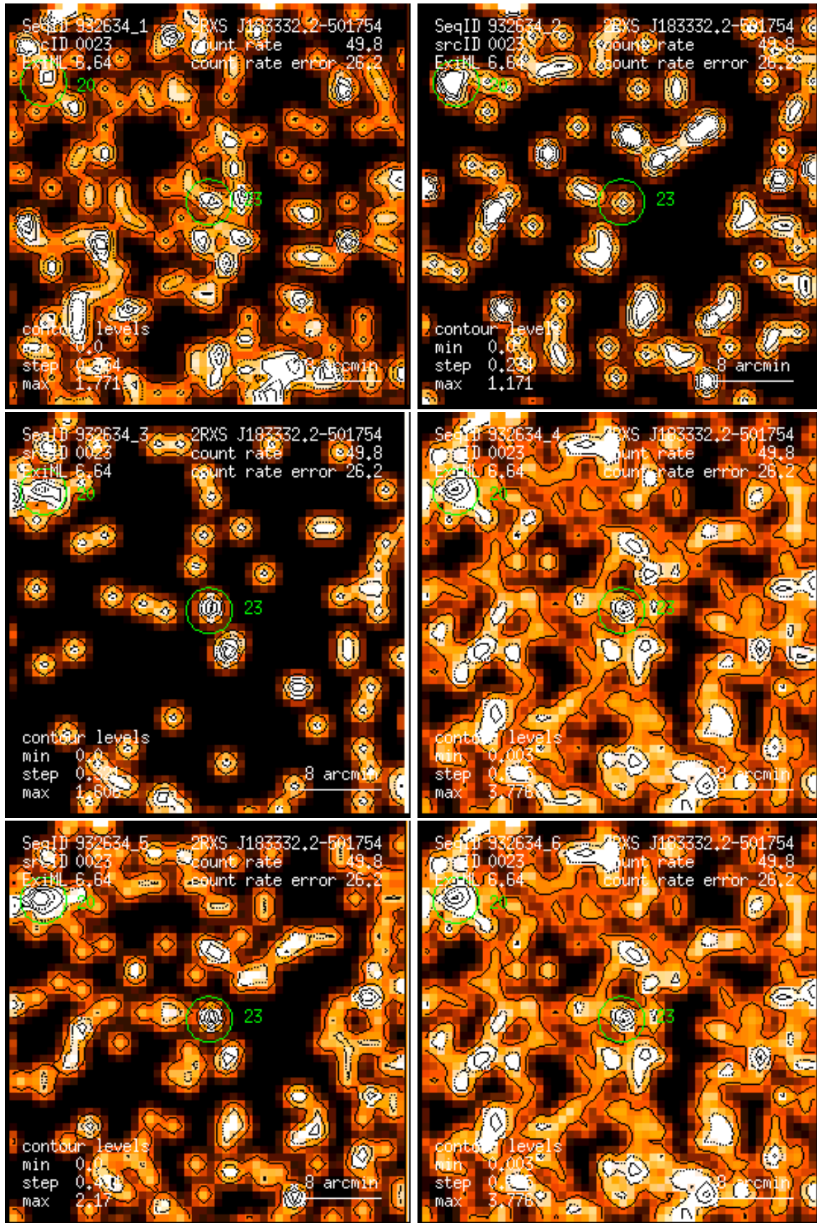
Figure 23: RASS 932634: detection 0023: band rate images, Gaussian filter: (1) PSPC channels 11 – 41, (2) 52 – 90, (3) 91 – 201, (4) 11 – 235, (5) 52 – 201, (6) 11 – 201. Broad band rates in counts/ks. Band rate contour levels in counts/ks/arcmin 2 .
