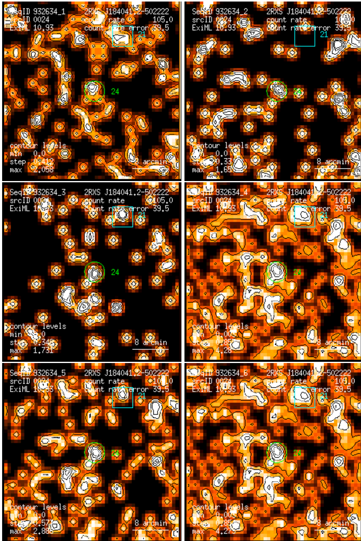
Figure 24: RASS 932634: detection 0024: band rate images, Gaussian filter: (1) PSPC channels 11 – 41, (2) 52 – 90, (3) 91 – 201, (4) 11 – 235, (5) 52 – 201, (6) 11 – 201. Broad band rates in counts/ks. Band rate contour levels in counts/ks/arcmin 2 .
