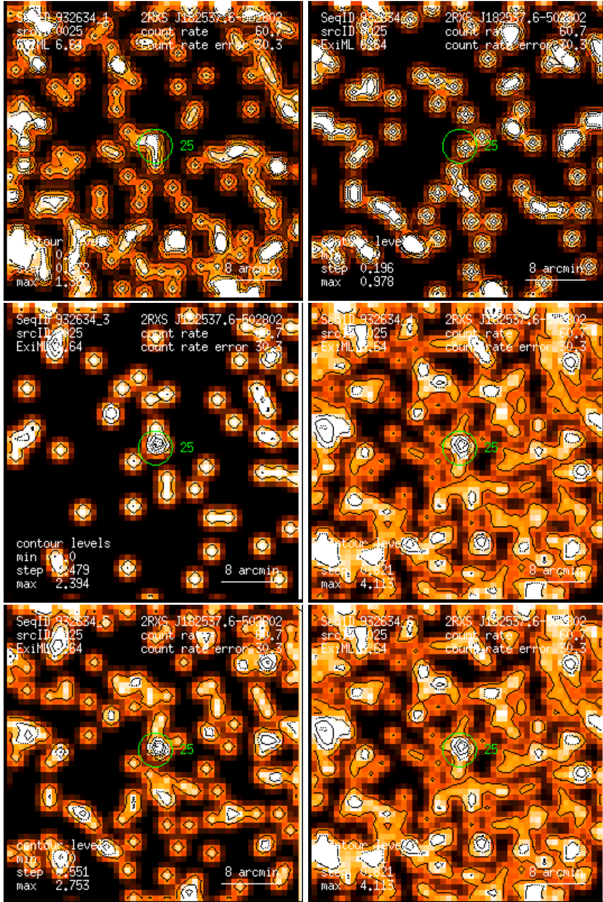
Figure 25: RASS 932634: detection 0025: band rate images, Gaussian filter: (1) PSPC channels 11 – 41, (2) 52 – 90, (3) 91 – 201, (4) 11 – 235, (5) 52 – 201, (6) 11 – 201. Broad band rates in counts/ks. Band rate contour levels in counts/ks/arcmin 2 .
