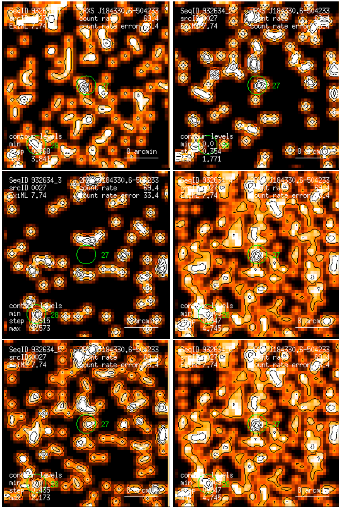
Figure 27: RASS 932634: detection 0027: band rate images, Gaussian filter: (1) PSPC channels 11 – 41, (2) 52 – 90, (3) 91 – 201, (4) 11 – 235, (5) 52 – 201, (6) 11 – 201. Broad band rates in counts/ks. Band rate contour levels in counts/ks/arcmin 2 .
