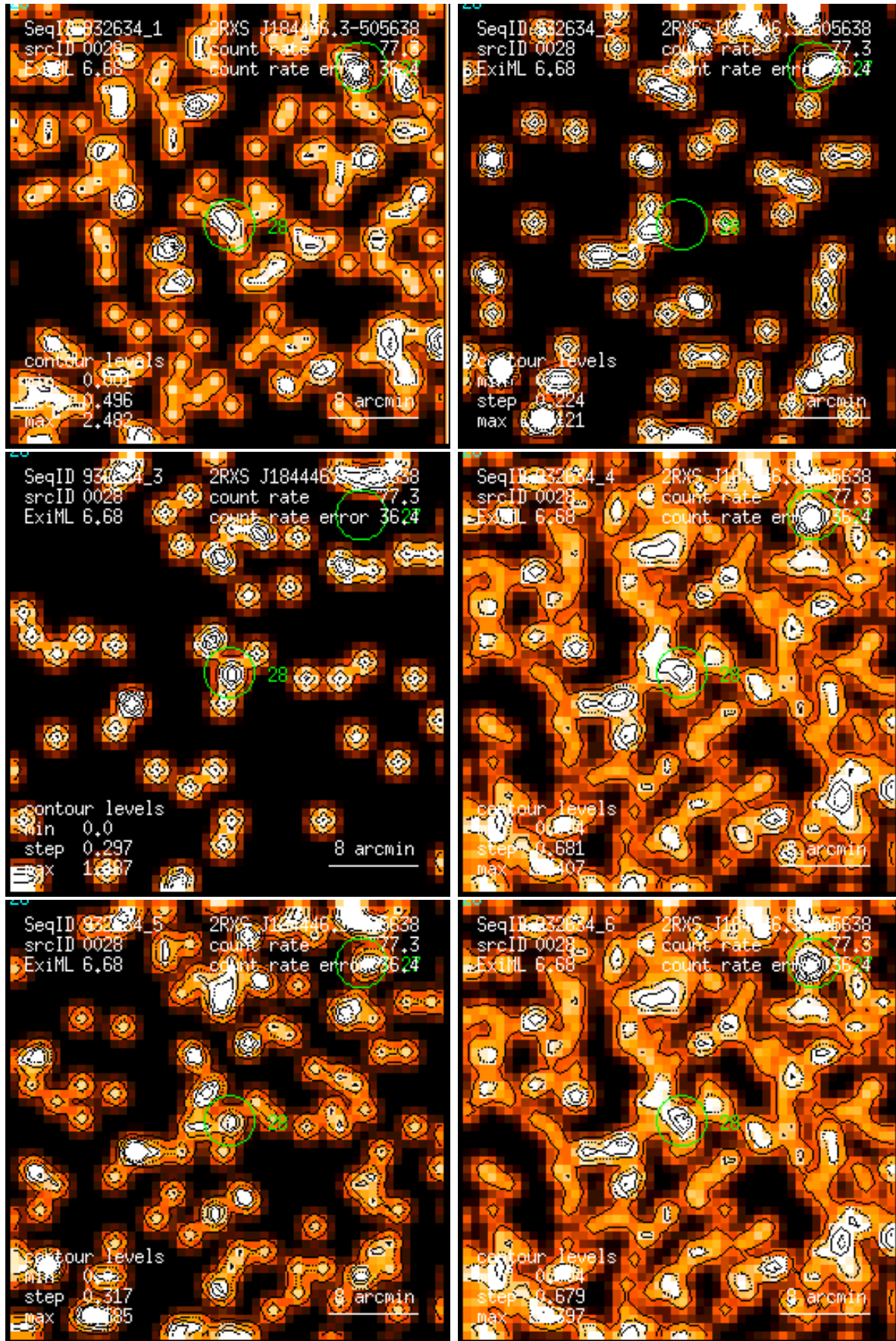
Figure 28: RASS 932634: detection 0028: band rate images, Gaussian filter: (1) PSPC channels 11 – 41, (2) 52 – 90, (3) 91 – 201, (4) 11 – 235, (5) 52 – 201, (6) 11 – 201. Broad band rates in counts/ks. Band rate contour levels in counts/ks/arcmin 2 .
