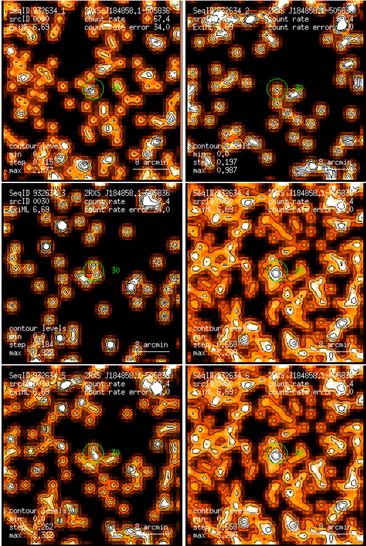
Figure 30: RASS 932634: detection 0030: band rate images, Gaussian filter: (1) PSPC channels 11 – 41, (2) 52 – 90, (3) 91 – 201, (4) 11 – 235, (5) 52 – 201, (6) 11 – 201. Broad band rates in counts/ks. Band rate contour levels in counts/ks/arcmin 2 .
