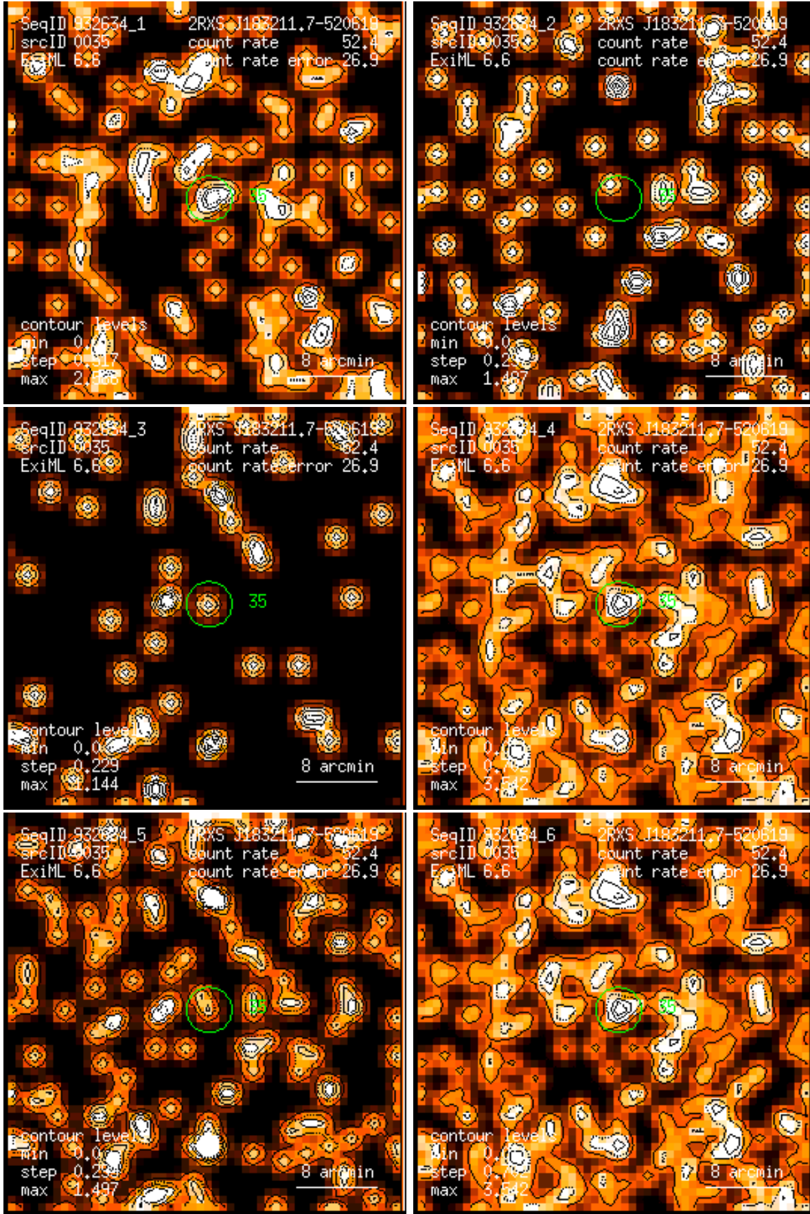
Figure 35: RASS 932634: detection 0035: band rate images, Gaussian filter: (1) PSPC channels 11 – 41, (2) 52 – 90, (3) 91 – 201, (4) 11 – 235, (5) 52 – 201, (6) 11 – 201. Broad band rates in counts/ks. Band rate contour levels in counts/ks/arcmin 2 .
