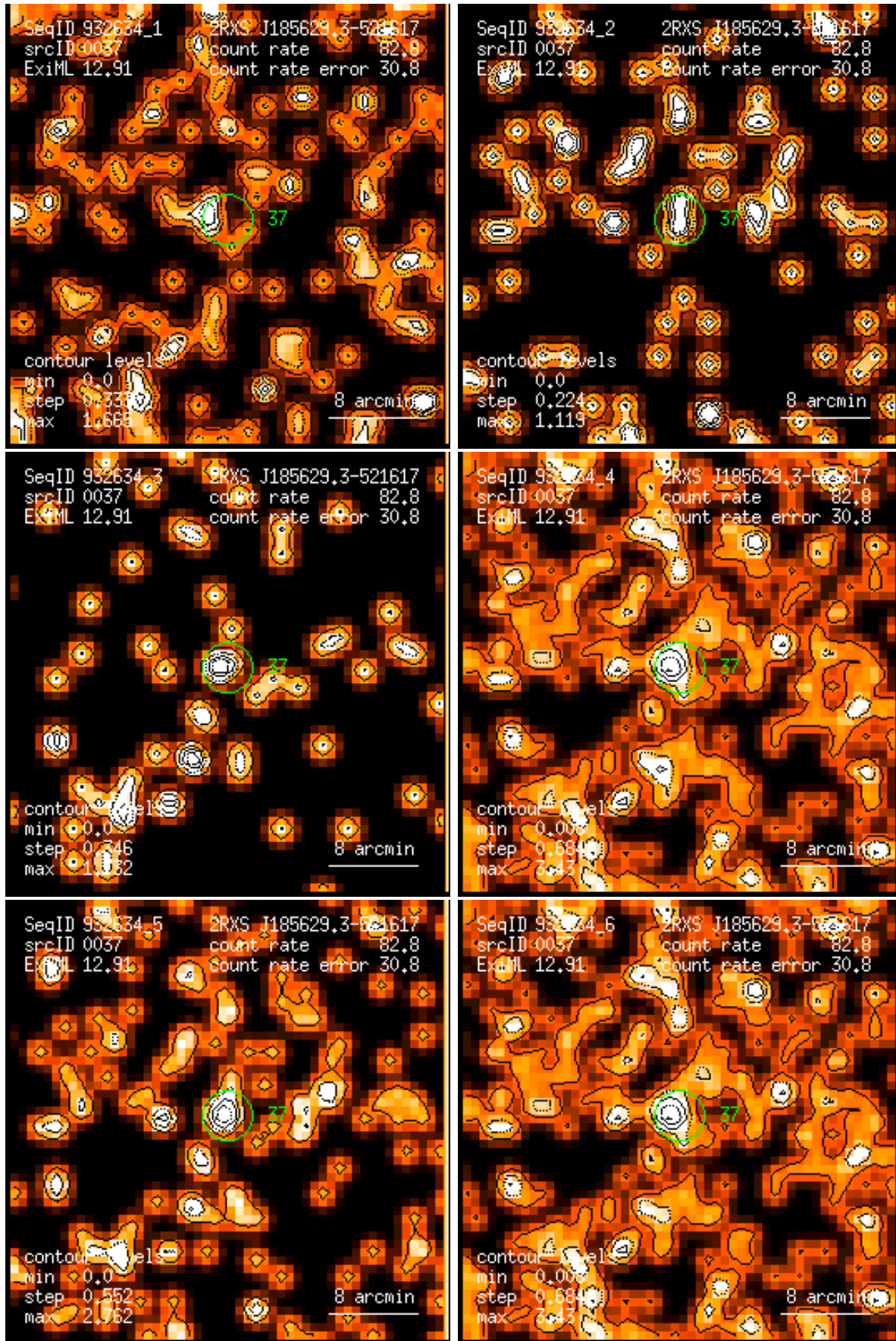
Figure 37: RASS 932634: detection 0037: band rate images, Gaussian filter: (1) PSPC channels 11 – 41, (2) 52 – 90, (3) 91 – 201, (4) 11 – 235, (5) 52 – 201, (6) 11 – 201. Broad band rates in counts/ks. Band rate contour levels in counts/ks/arcmin 2 .
