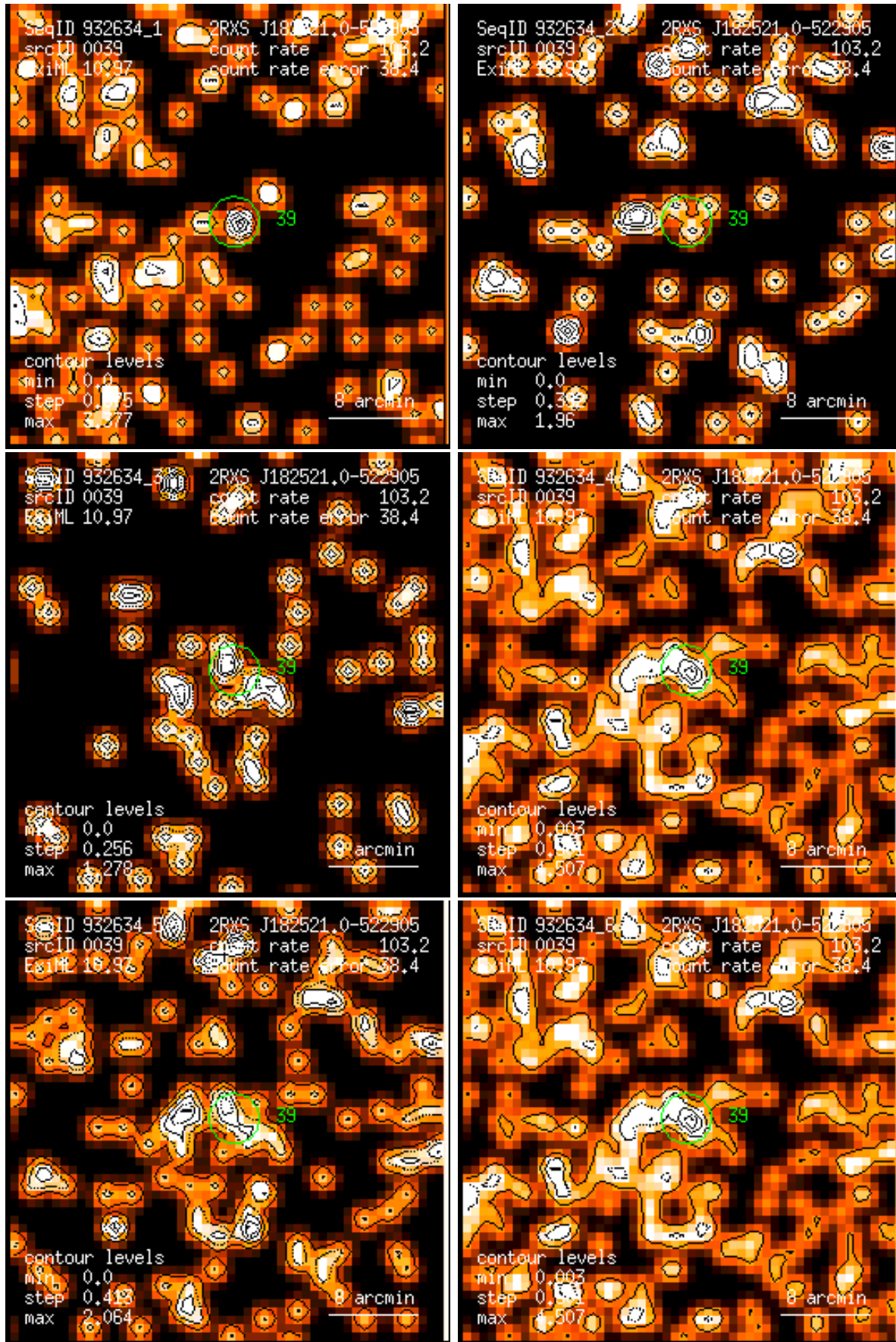
Figure 39: RASS 932634: detection 0039: band rate images, Gaussian filter: (1) PSPC channels 11 – 41, (2) 52 – 90, (3) 91 – 201, (4) 11 – 235, (5) 52 – 201, (6) 11 – 201. Broad band rates in counts/ks. Band rate contour levels in counts/ks/arcmin 2 .
