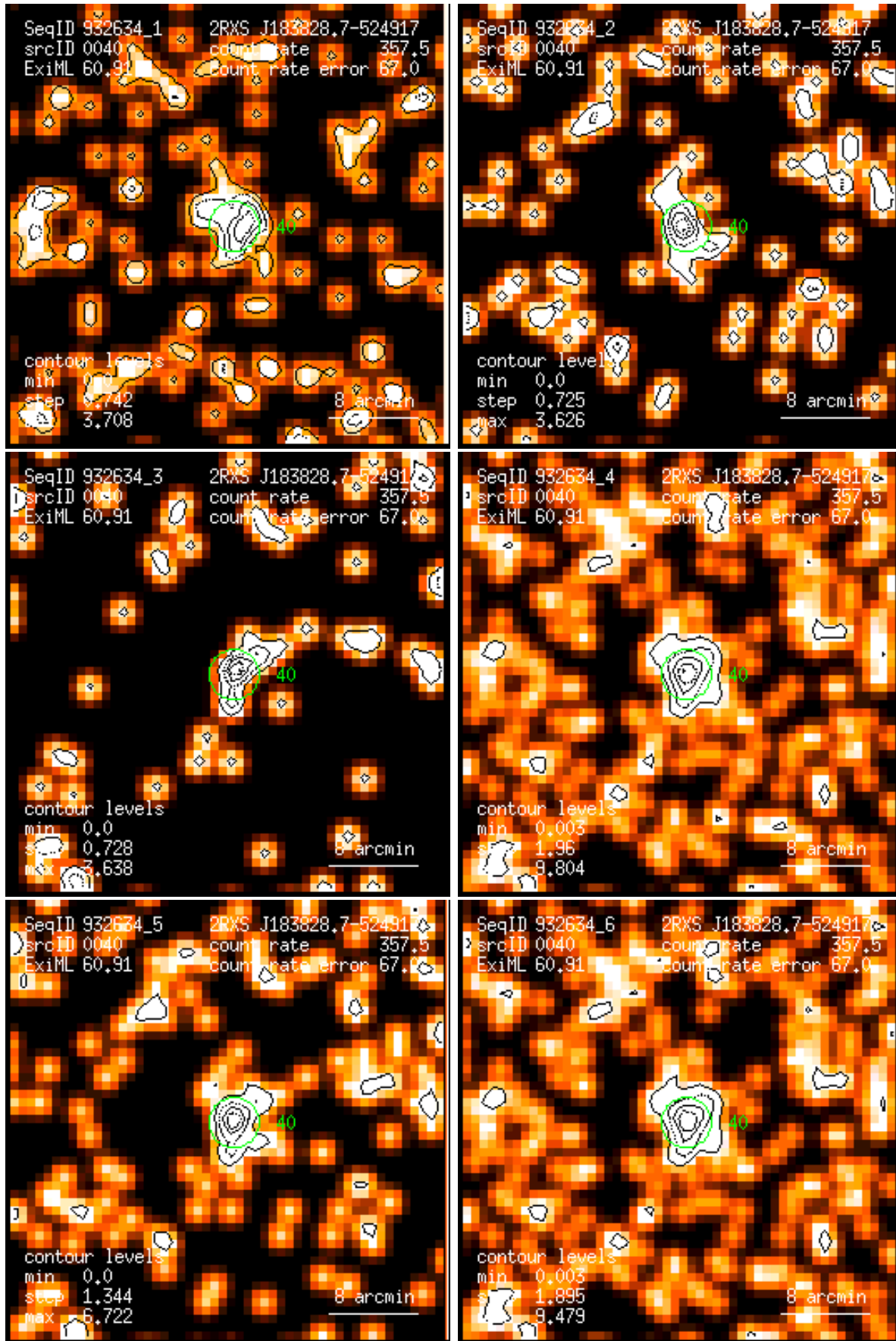
Figure 40: RASS 932634: detection 0040: band rate images, Gaussian filter: (1) PSPC channels 11 – 41, (2) 52 – 90, (3) 91 – 201, (4) 11 – 235, (5) 52 – 201, (6) 11 – 201. Broad band rates in counts/ks. Band rate contour levels in counts/ks/arcmin 2 .
