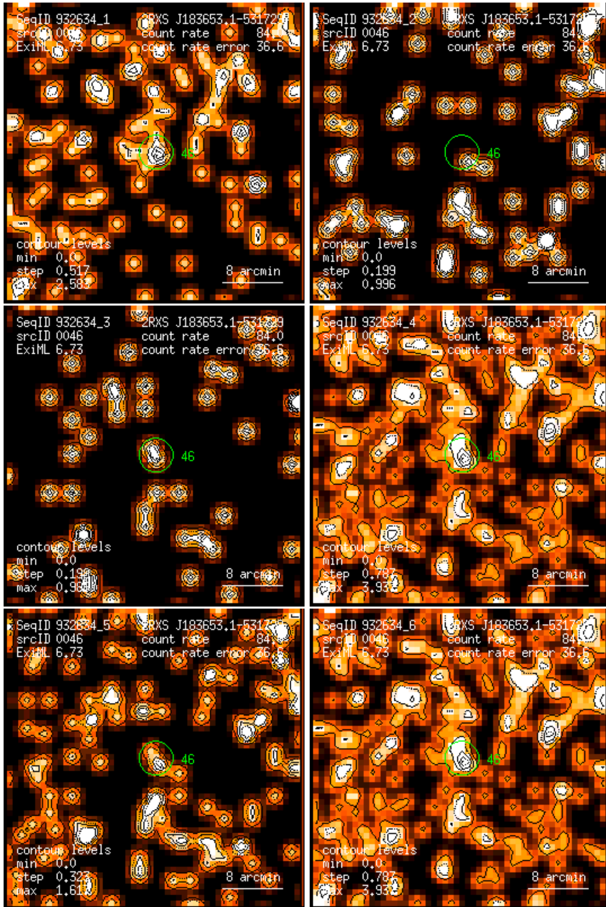
Figure 46: RASS 932634: detection 0046: band rate images, Gaussian filter: (1) PSPC channels 11 – 41, (2) 52 – 90, (3) 91 – 201, (4) 11 – 235, (5) 52 – 201, (6) 11 – 201. Broad band rates in counts/ks. Band rate contour levels in counts/ks/arcmin 2 .
