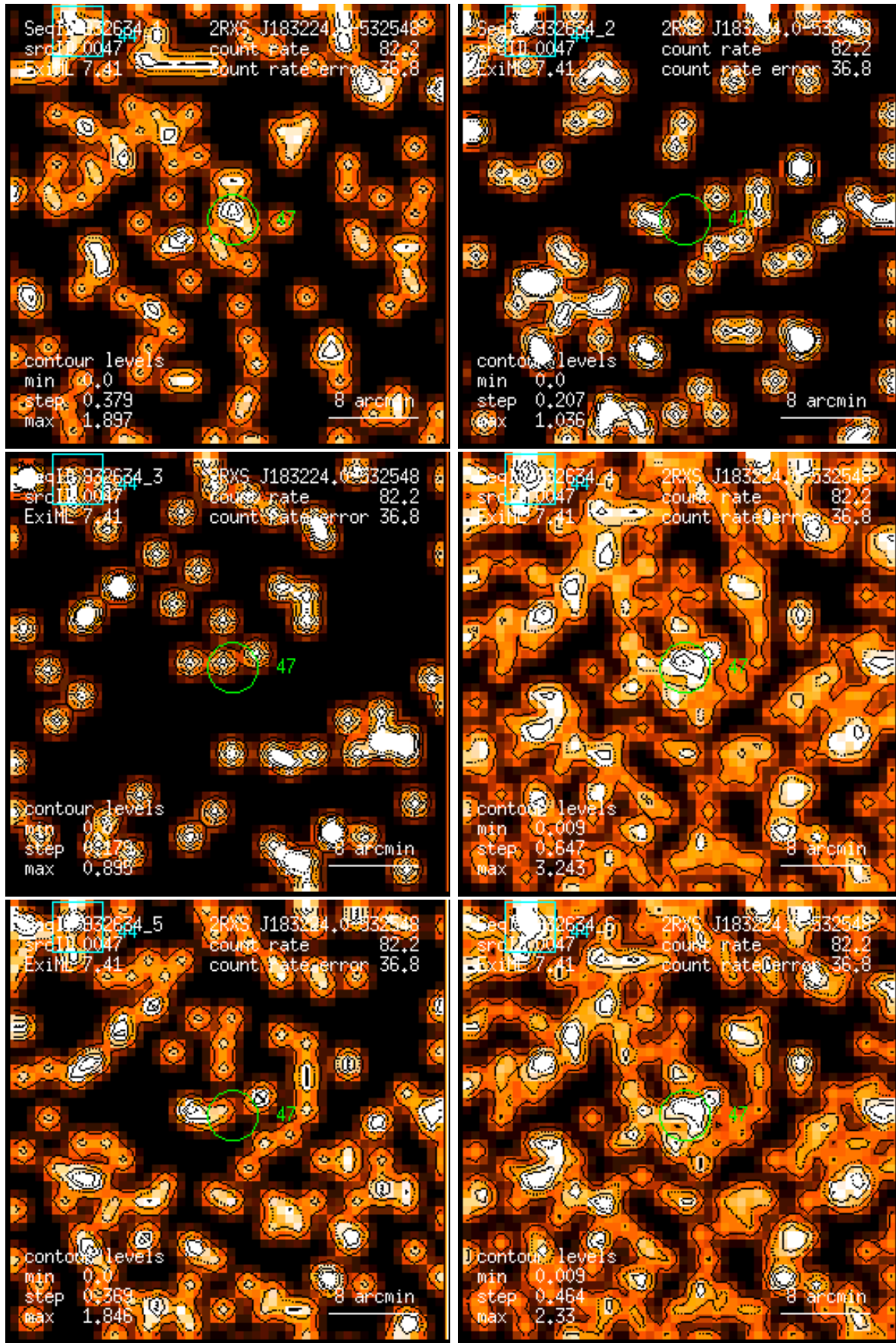
Figure 47: RASS 932634: detection 0047: band rate images, Gaussian filter: (1) PSPC channels 11 – 41, (2) 52 – 90, (3) 91 – 201, (4) 11 – 235, (5) 52 – 201, (6) 11 – 201. Broad band rates in counts/ks. Band rate contour levels in counts/ks/arcmin 2 .
