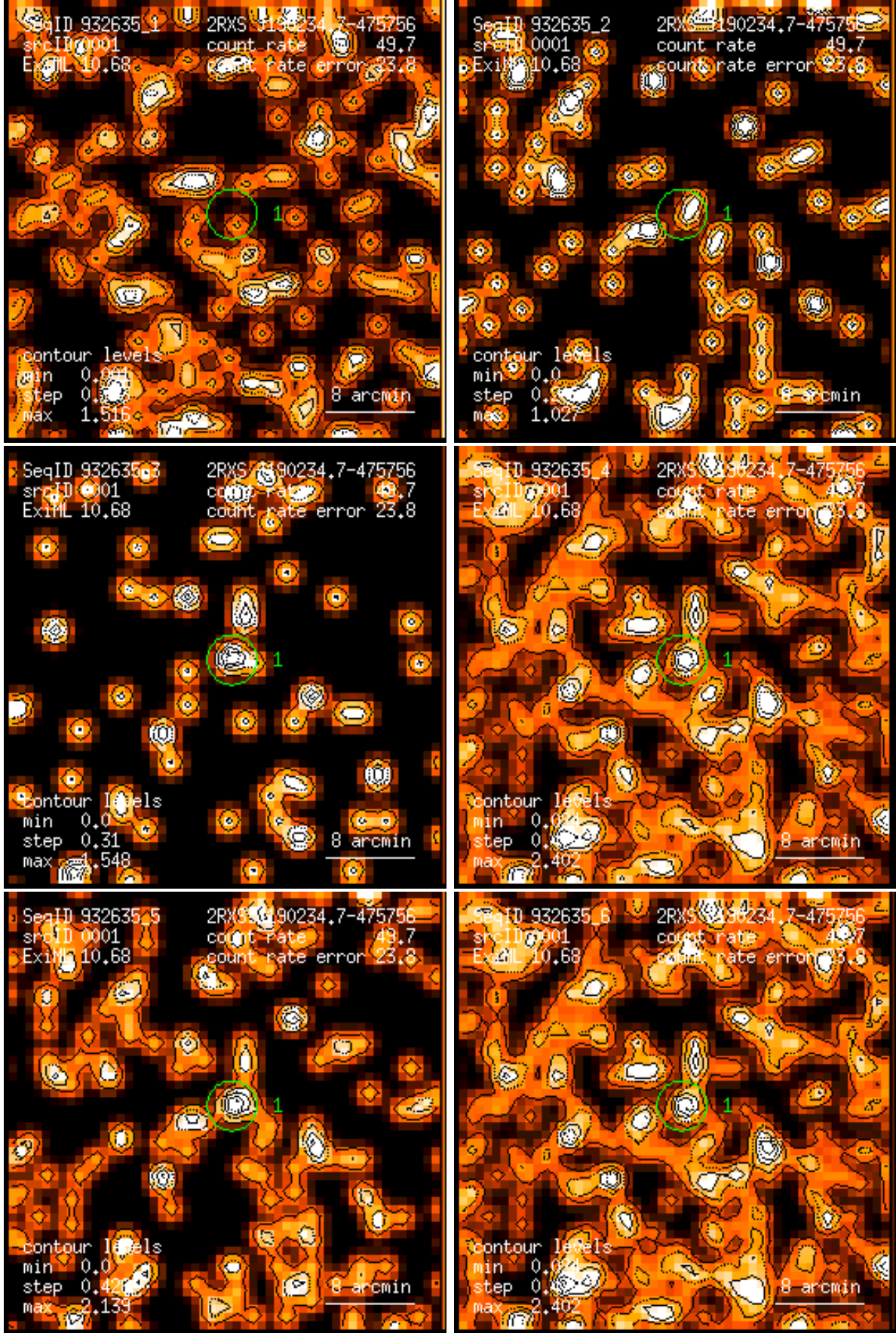
Figure 1: RASS 932635: detection 0001: band rate images, Gaussian filter: (1) PSPC channels 11 – 41, (2) 52 – 90, (3) 91 – 201, (4) 11 – 235, (5) 52 – 201, (6) 11 – 201. Broad band rates in counts/ks. Band rate contour levels in counts/ks/arcmin 2 .
