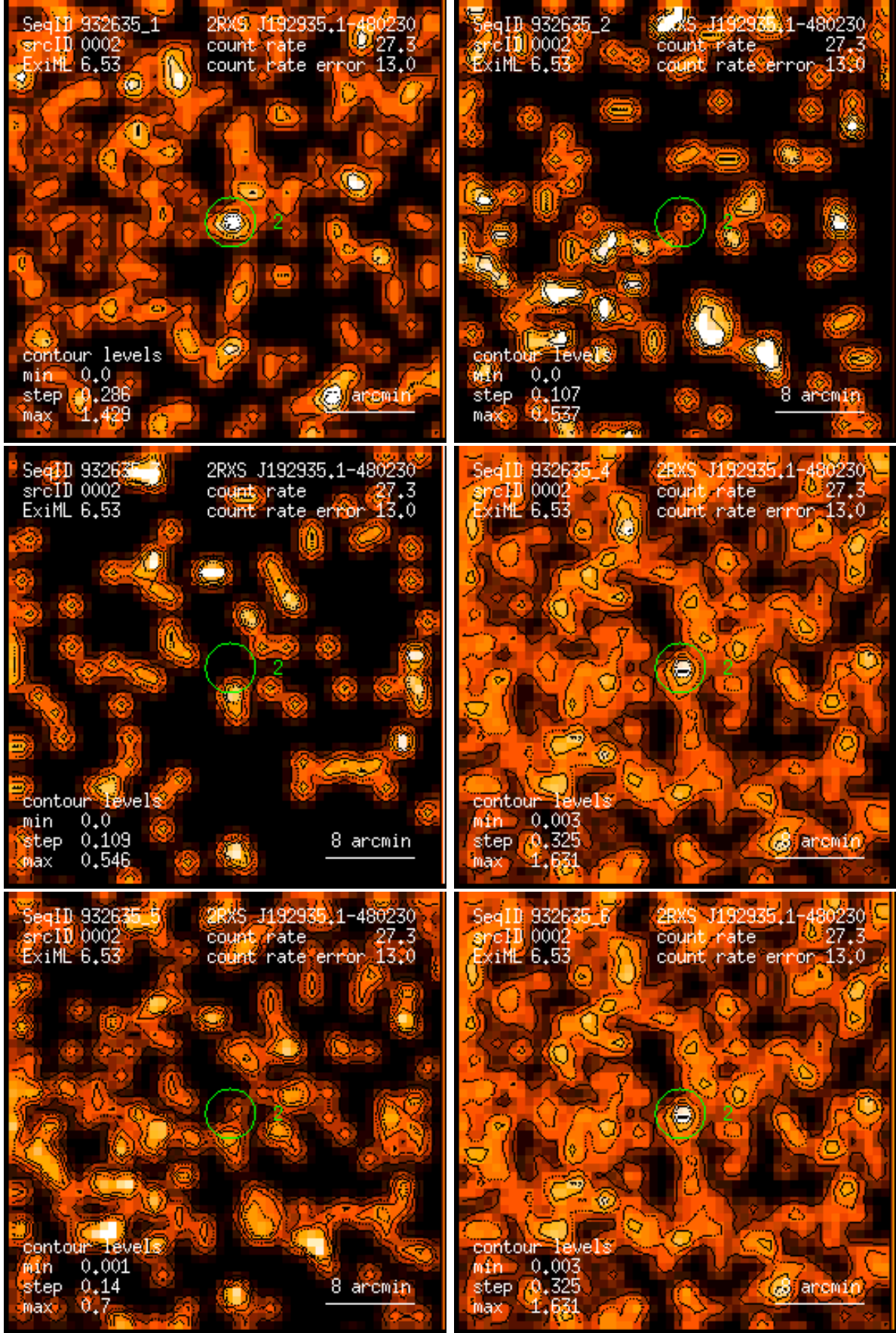
Figure 2: RASS 932635: detection 0002: band rate images, Gaussian filter: (1) PSPC channels 11 – 41, (2) 52 – 90, (3) 91 – 201, (4) 11 – 235, (5) 52 – 201, (6) 11 – 201. Broad band rates in counts/ks. Band rate contour levels in counts/ks/arcmin 2 .
