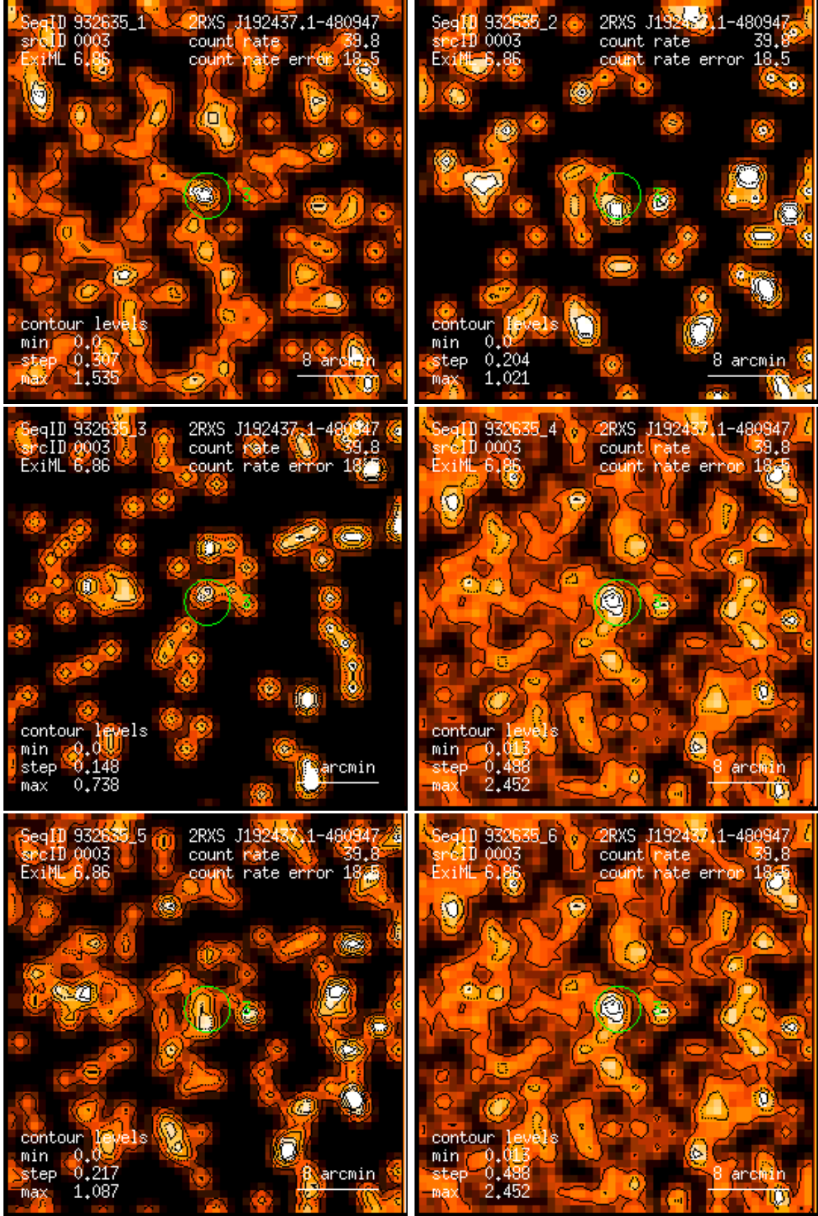
Figure 3: RASS 932635: detection 0003: band rate images, Gaussian filter: (1) PSPC channels 11 – 41, (2) 52 – 90, (3) 91 – 201, (4) 11 – 235, (5) 52 – 201, (6) 11 – 201. Broad band rates in counts/ks. Band rate contour levels in counts/ks/arcmin 2 .
