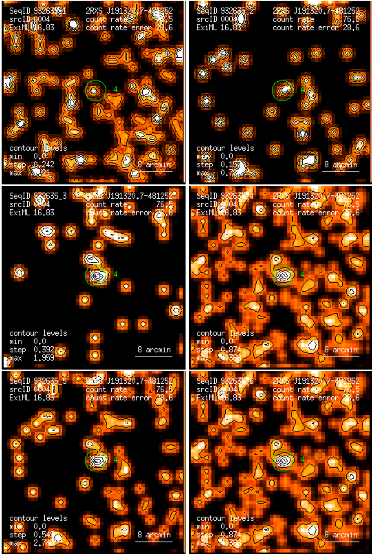
Figure 4: RASS 932635: detection 0004: band rate images, Gaussian filter: (1) PSPC channels 11 – 41, (2) 52 – 90, (3) 91 – 201, (4) 11 – 235, (5) 52 – 201, (6) 11 – 201. Broad band rates in counts/ks. Band rate contour levels in counts/ks/arcmin 2 .
