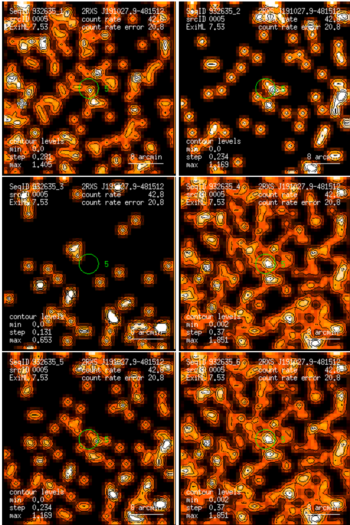
Figure 5: RASS 932635: detection 0005: band rate images, Gaussian filter: (1) PSPC channels 11 – 41, (2) 52 – 90, (3) 91 – 201, (4) 11 – 235, (5) 52 – 201, (6) 11 – 201. Broad band rates in counts/ks. Band rate contour levels in counts/ks/arcmin 2 .
