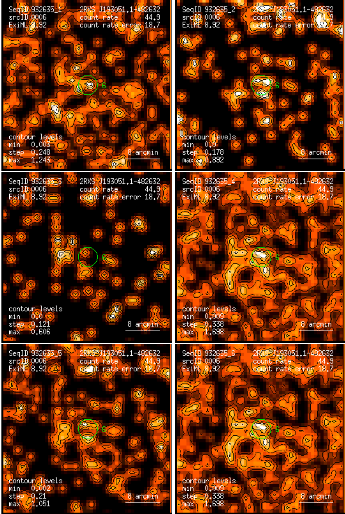
Figure 6: RASS 932635: detection 0006: band rate images, Gaussian filter: (1) PSPC channels 11 – 41, (2) 52 – 90, (3) 91 – 201, (4) 11 – 235, (5) 52 – 201, (6) 11 – 201. Broad band rates in counts/ks. Band rate contour levels in counts/ks/arcmin 2 .
