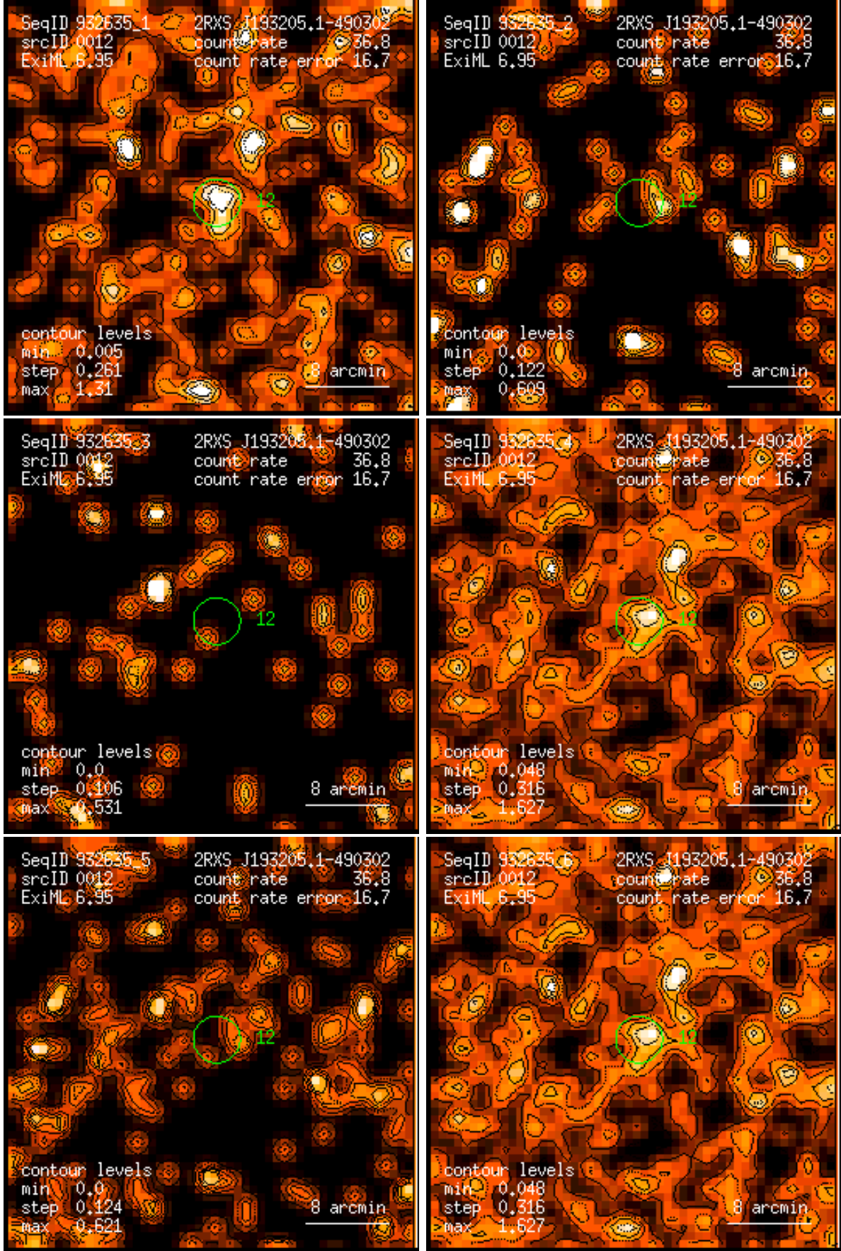
Figure 12: RASS 932635: detection 0012: band rate images, Gaussian filter: (1) PSPC channels 11 – 41, (2) 52 – 90, (3) 91 – 201, (4) 11 – 235, (5) 52 – 201, (6) 11 – 201. Broad band rates in counts/ks. Band rate contour levels in counts/ks/arcmin 2 .
