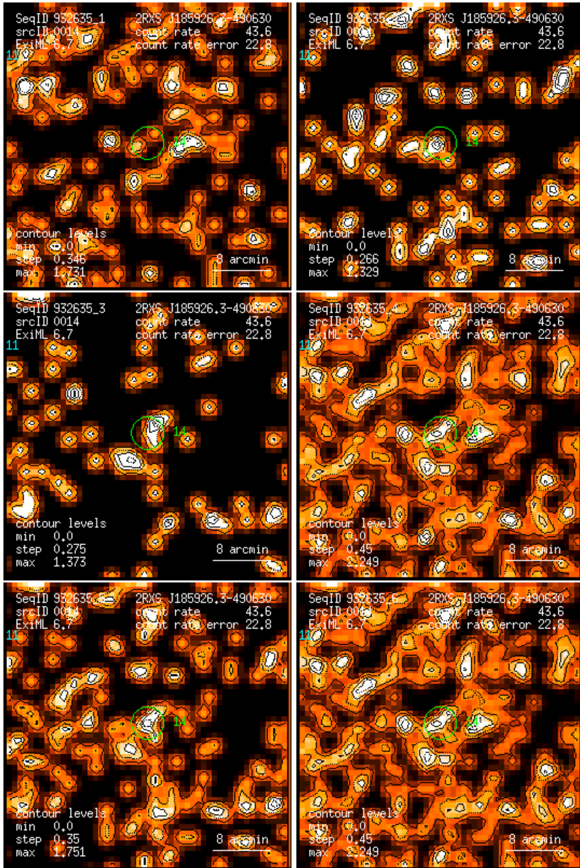
Figure 14: RASS 932635: detection 0014: band rate images, Gaussian filter: (1) PSPC channels 11 – 41, (2) 52 – 90, (3) 91 – 201, (4) 11 – 235, (5) 52 – 201, (6) 11 – 201. Broad band rates in counts/ks. Band rate contour levels in counts/ks/arcmin 2 .
