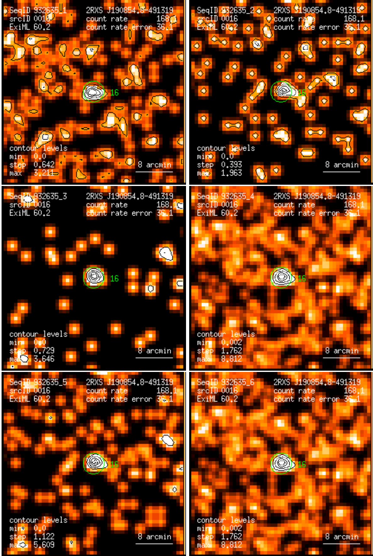
Figure 16: RASS 932635: detection 0016: band rate images, Gaussian filter: (1) PSPC channels 11 – 41, (2) 52 – 90, (3) 91 – 201, (4) 11 – 235, (5) 52 – 201, (6) 11 – 201. Broad band rates in counts/ks. Band rate contour levels in counts/ks/arcmin 2 .
