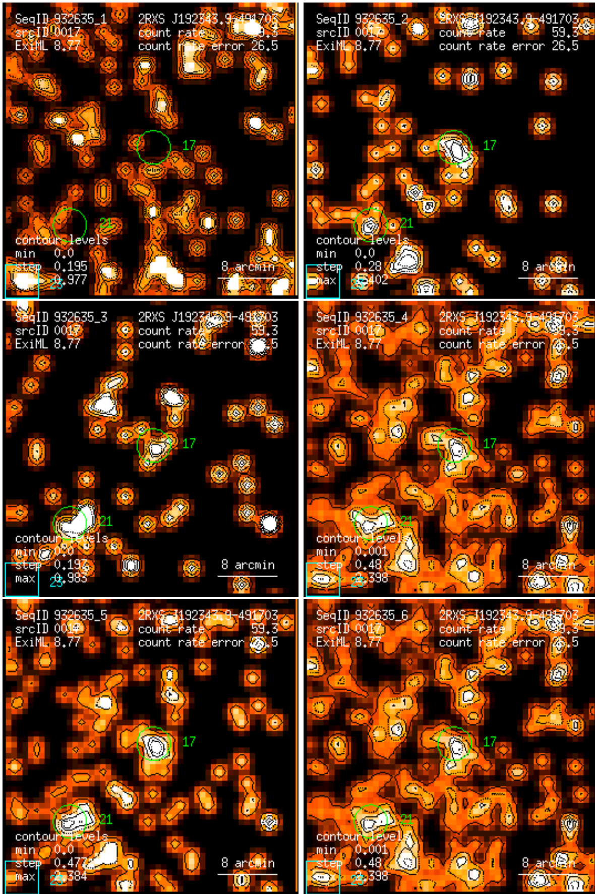
Figure 17: RASS 932635: detection 0017: band rate images, Gaussian filter: (1) PSPC channels 11 – 41, (2) 52 – 90, (3) 91 – 201, (4) 11 – 235, (5) 52 – 201, (6) 11 – 201. Broad band rates in counts/ks. Band rate contour levels in counts/ks/arcmin 2 .
