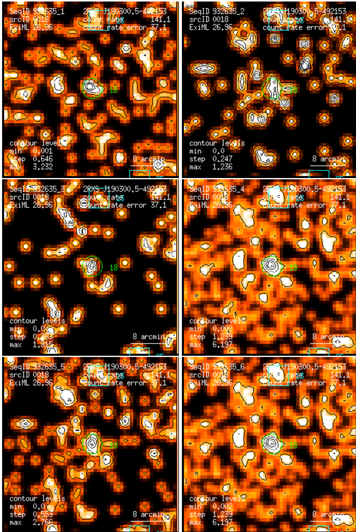
Figure 18: RASS 932635: detection 0018: band rate images, Gaussian filter: (1) PSPC channels 11 – 41, (2) 52 – 90, (3) 91 – 201, (4) 11 – 235, (5) 52 – 201, (6) 11 – 201. Broad band rates in counts/ks. Band rate contour levels in counts/ks/arcmin 2 .
