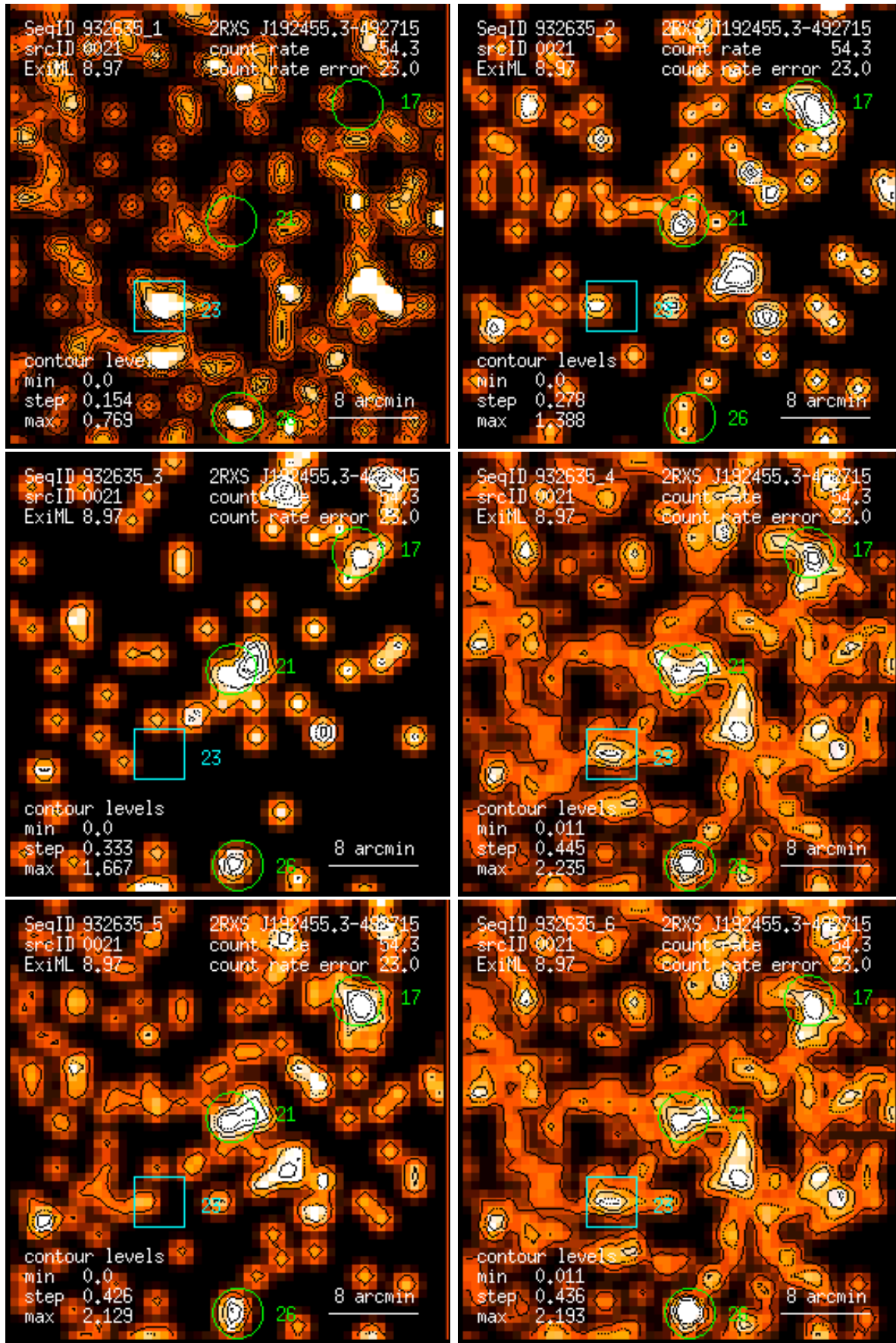
Figure 21: RASS 932635: detection 0021: band rate images, Gaussian filter: (1) PSPC channels 11 – 41, (2) 52 – 90, (3) 91 – 201, (4) 11 – 235, (5) 52 – 201, (6) 11 – 201. Broad band rates in counts/ks. Band rate contour levels in counts/ks/arcmin 2 .
