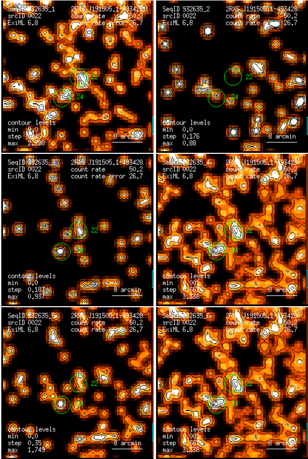
Figure 22: RASS 932635: detection 0022: band rate images, Gaussian filter: (1) PSPC channels 11 – 41, (2) 52 – 90, (3) 91 – 201, (4) 11 – 235, (5) 52 – 201, (6) 11 – 201. Broad band rates in counts/ks. Band rate contour levels in counts/ks/arcmin 2 .
