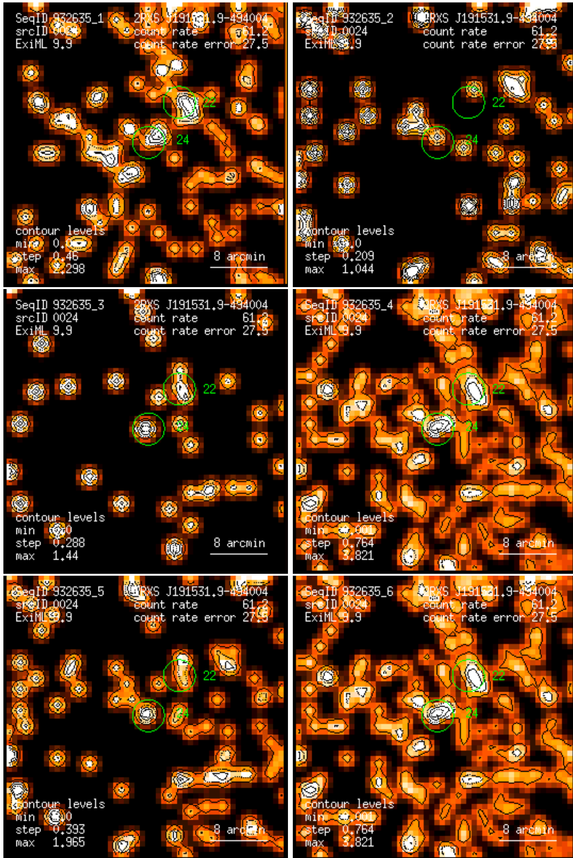
Figure 24: RASS 932635: detection 0024: band rate images, Gaussian filter: (1) PSPC channels 11 – 41, (2) 52 – 90, (3) 91 – 201, (4) 11 – 235, (5) 52 – 201, (6) 11 – 201. Broad band rates in counts/ks. Band rate contour levels in counts/ks/arcmin 2 .
