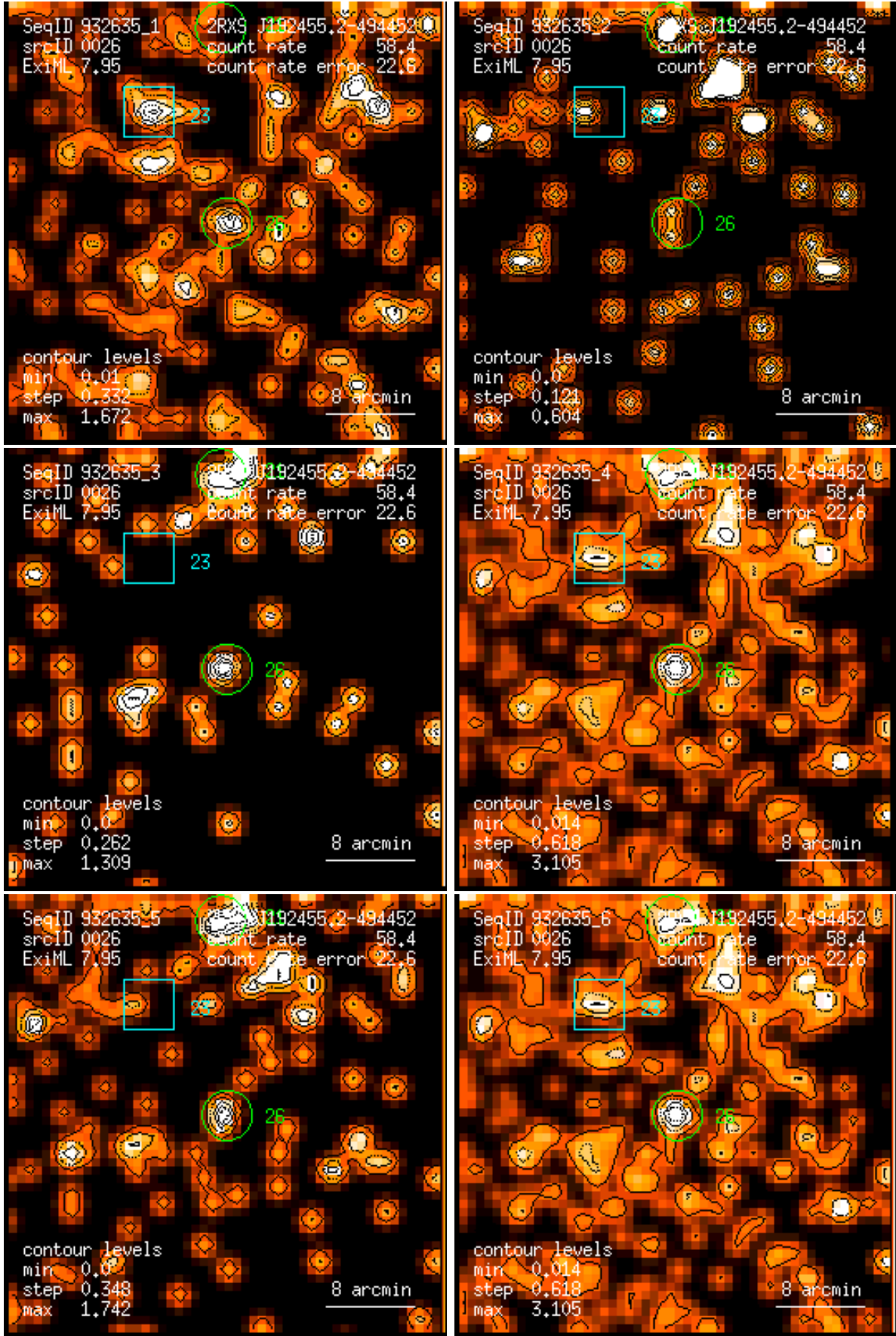
Figure 26: RASS 932635: detection 0026: band rate images, Gaussian filter: (1) PSPC channels 11 – 41, (2) 52 – 90, (3) 91 – 201, (4) 11 – 235, (5) 52 – 201, (6) 11 – 201. Broad band rates in counts/ks. Band rate contour levels in counts/ks/arcmin 2 .
