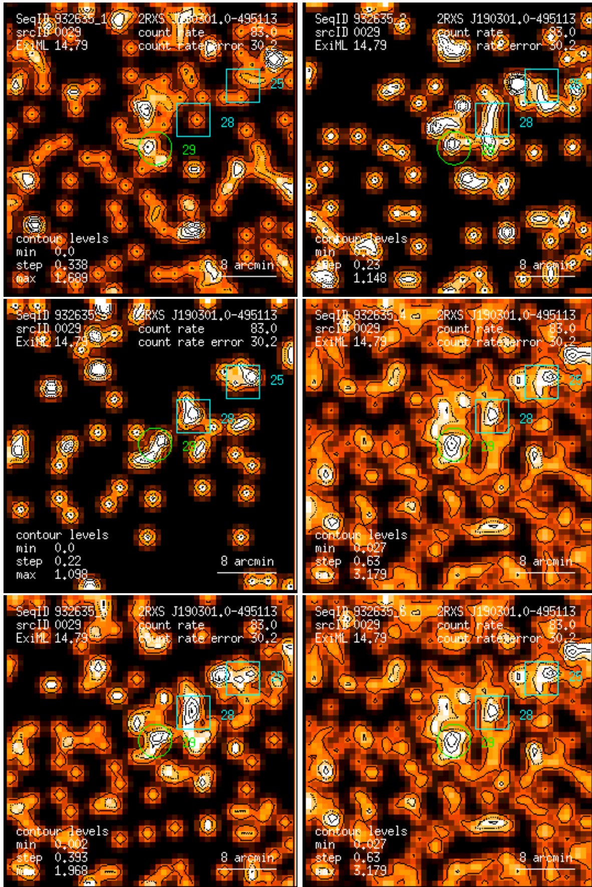
Figure 29: RASS 932635: detection 0029: band rate images, Gaussian filter: (1) PSPC channels 11 – 41, (2) 52 – 90, (3) 91 – 201, (4) 11 – 235, (5) 52 – 201, (6) 11 – 201. Broad band rates in counts/ks. Band rate contour levels in counts/ks/arcmin 2 .
