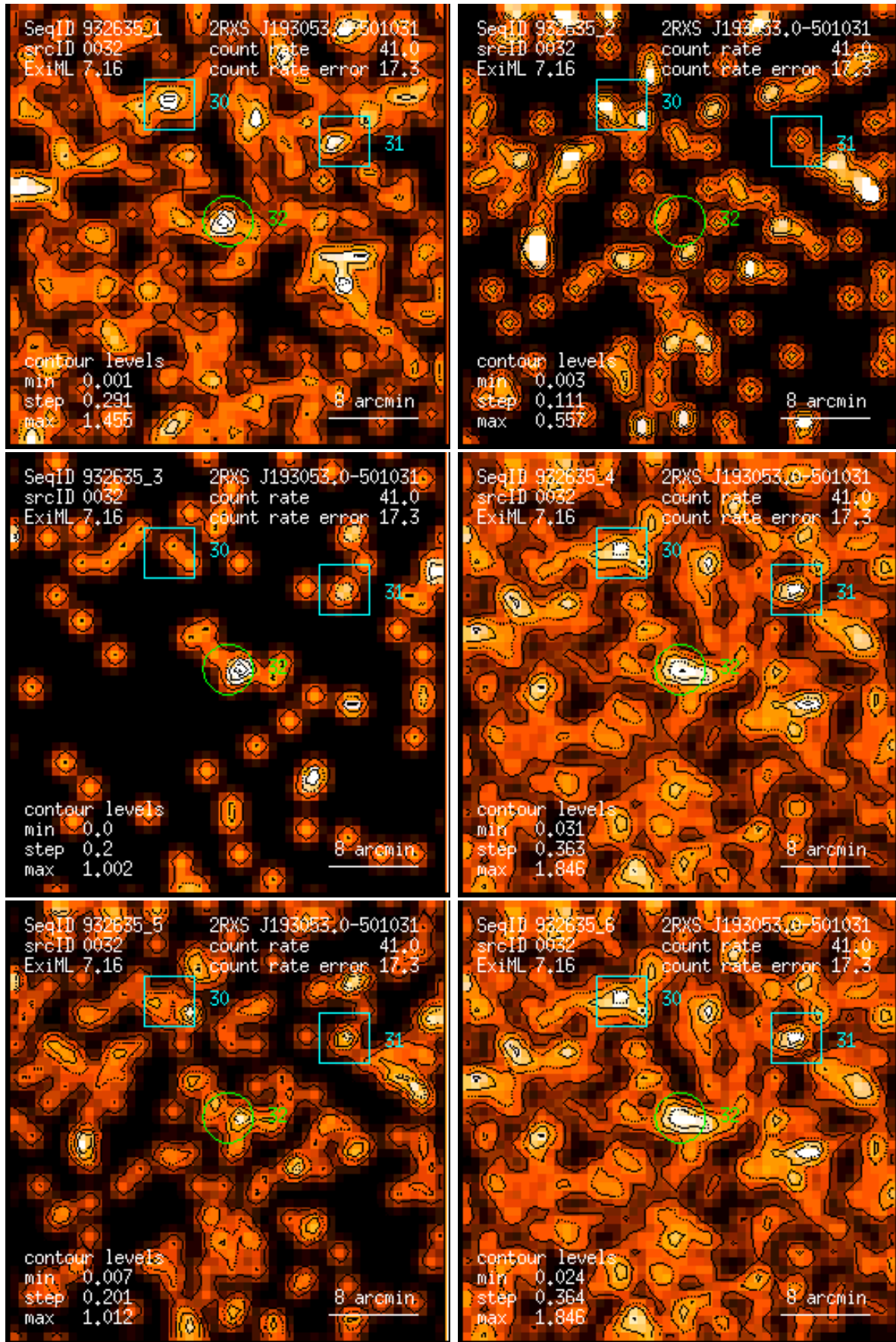
Figure 32: RASS 932635: detection 0032: band rate images, Gaussian filter: (1) PSPC channels 11 – 41, (2) 52 – 90, (3) 91 – 201, (4) 11 – 235, (5) 52 – 201, (6) 11 – 201. Broad band rates in counts/ks. Band rate contour levels in counts/ks/arcmin 2 .
