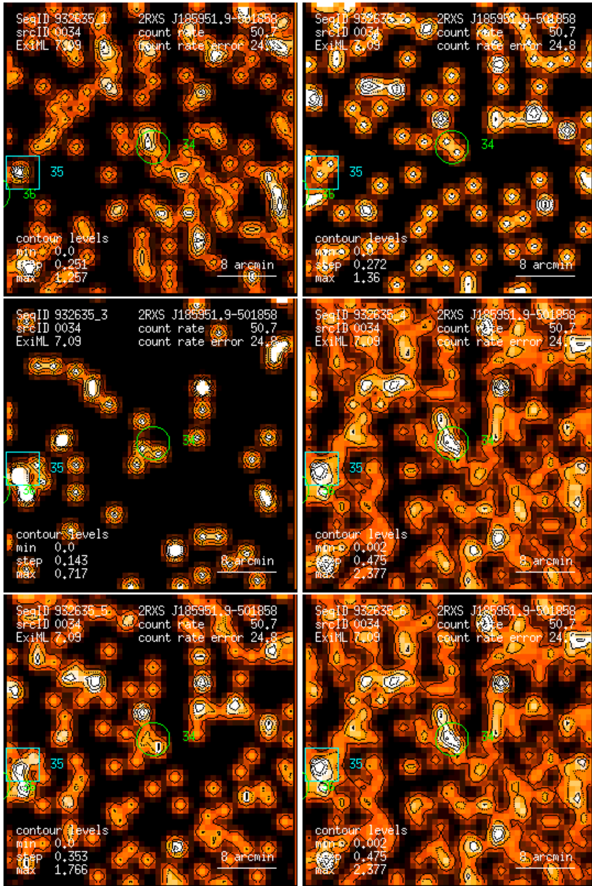
Figure 34: RASS 932635: detection 0034: band rate images, Gaussian filter: (1) PSPC channels 11 – 41, (2) 52 – 90, (3) 91 – 201, (4) 11 – 235, (5) 52 – 201, (6) 11 – 201. Broad band rates in counts/ks. Band rate contour levels in counts/ks/arcmin 2 .
