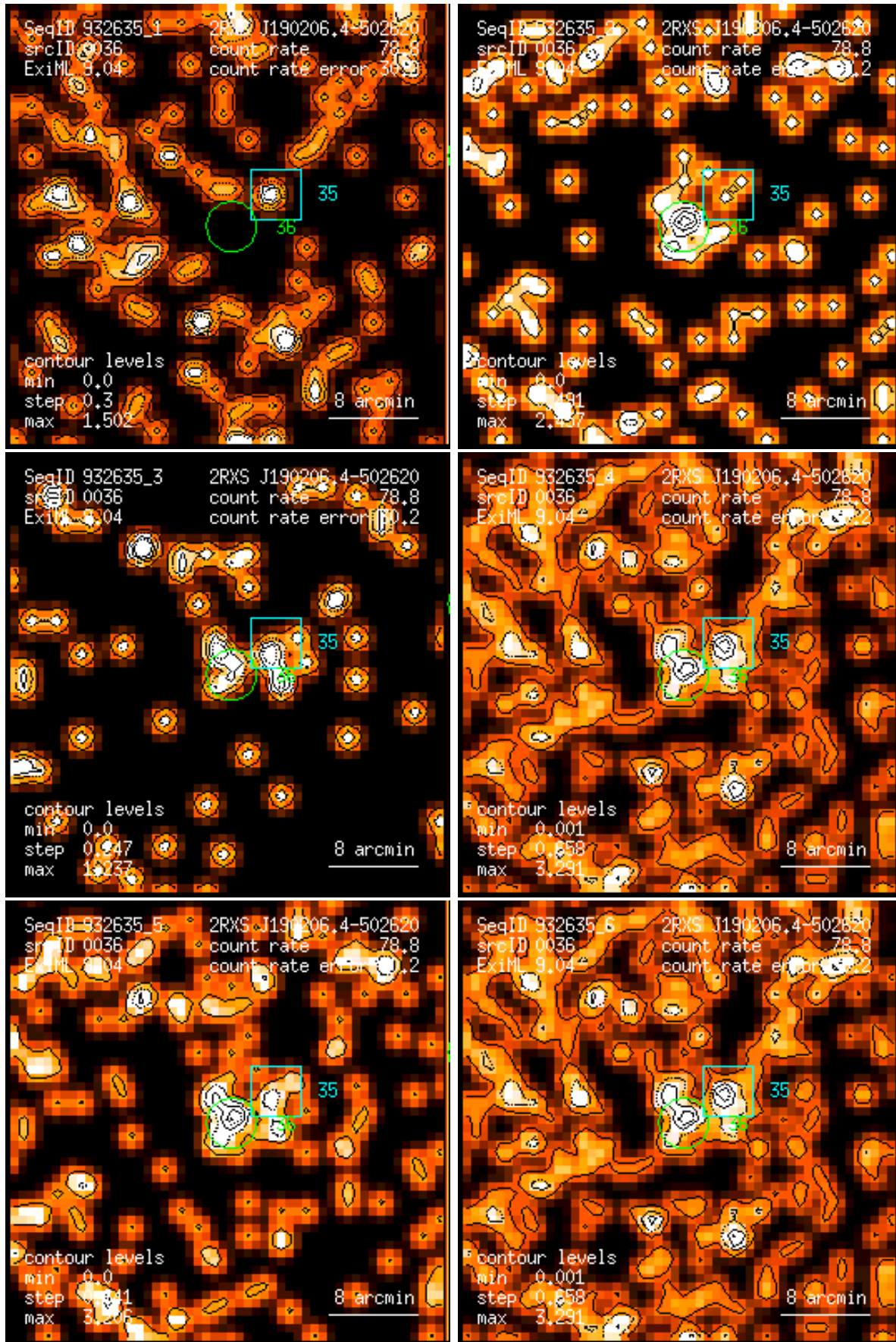
Figure 36: RASS 932635: detection 0036: band rate images, Gaussian filter: (1) PSPC channels 11 – 41, (2) 52 – 90, (3) 91 – 201, (4) 11 – 235, (5) 52 – 201, (6) 11 – 201. Broad band rates in counts/ks. Band rate contour levels in counts/ks/arcmin 2 .
