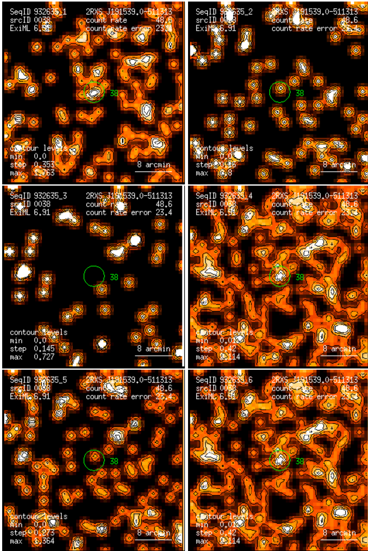
Figure 38: RASS 932635: detection 0038: band rate images, Gaussian filter: (1) PSPC channels 11 – 41, (2) 52 – 90, (3) 91 – 201, (4) 11 – 235, (5) 52 – 201, (6) 11 – 201. Broad band rates in counts/ks. Band rate contour levels in counts/ks/arcmin 2 .
