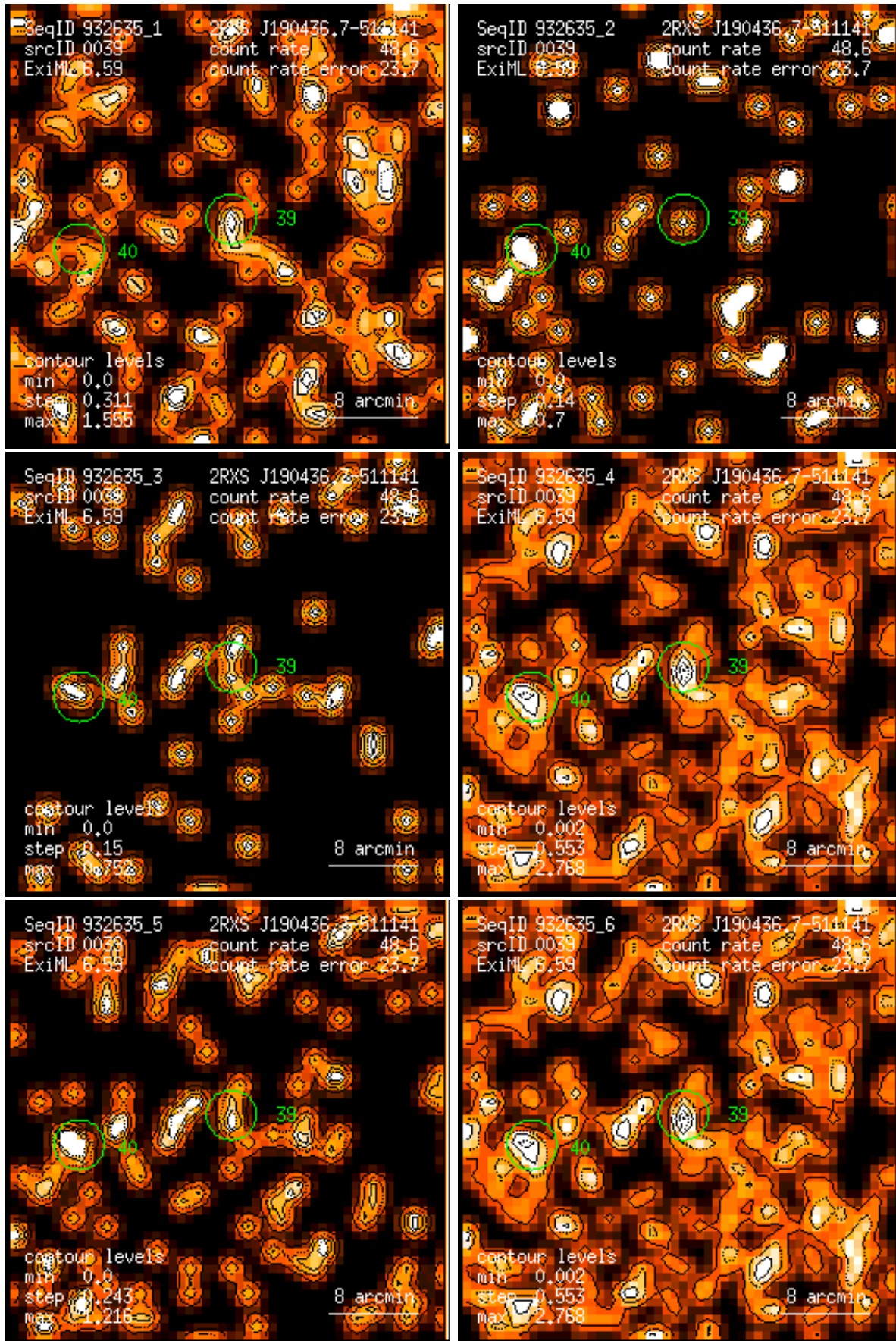
Figure 39: RASS 932635: detection 0039: band rate images, Gaussian filter: (1) PSPC channels 11 – 41, (2) 52 – 90, (3) 91 – 201, (4) 11 – 235, (5) 52 – 201, (6) 11 – 201. Broad band rates in counts/ks. Band rate contour levels in counts/ks/arcmin 2 .
