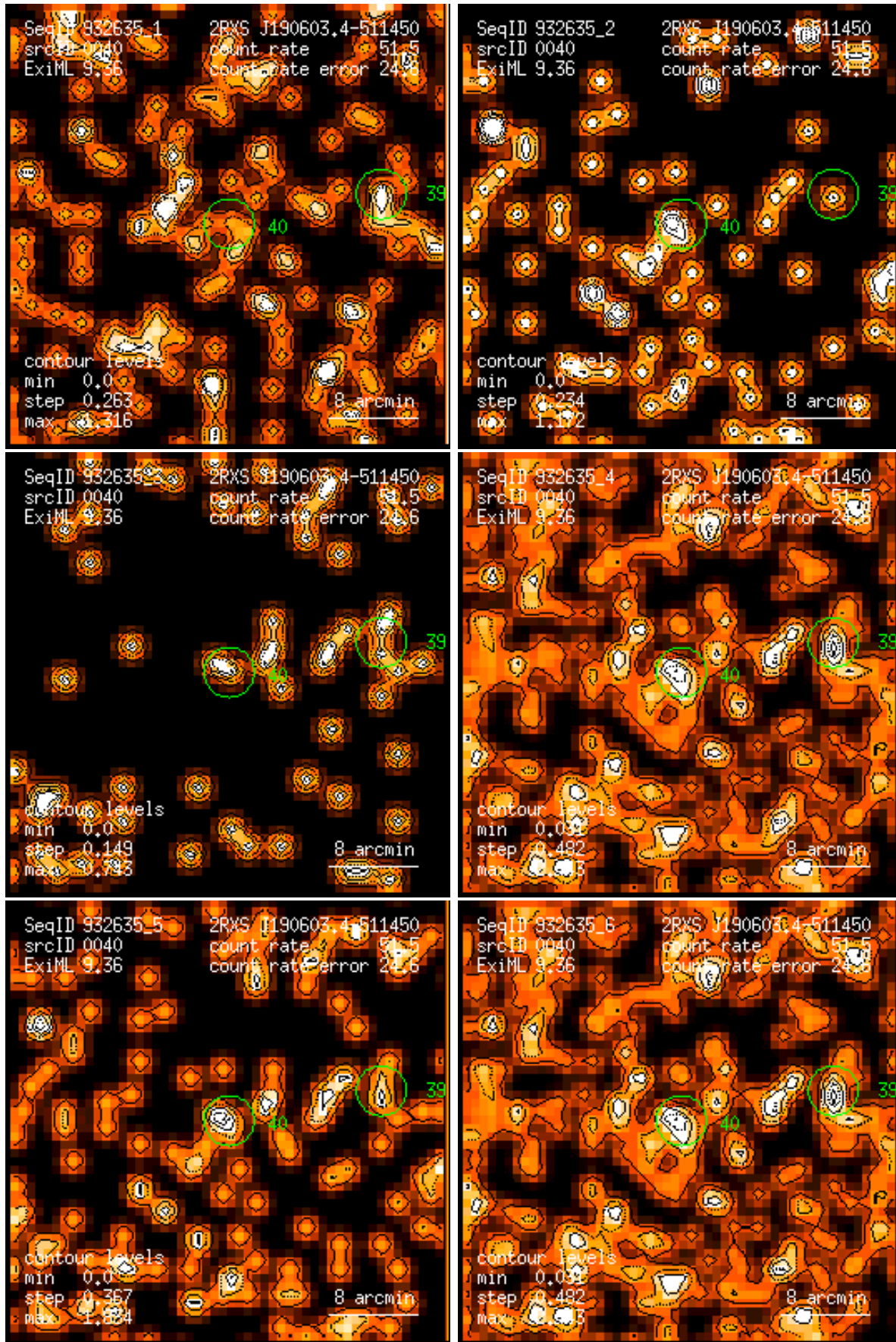
Figure 40: RASS 932635: detection 0040: band rate images, Gaussian filter: (1) PSPC channels 11 – 41, (2) 52 – 90, (3) 91 – 201, (4) 11 – 235, (5) 52 – 201, (6) 11 – 201. Broad band rates in counts/ks. Band rate contour levels in counts/ks/arcmin 2 .
