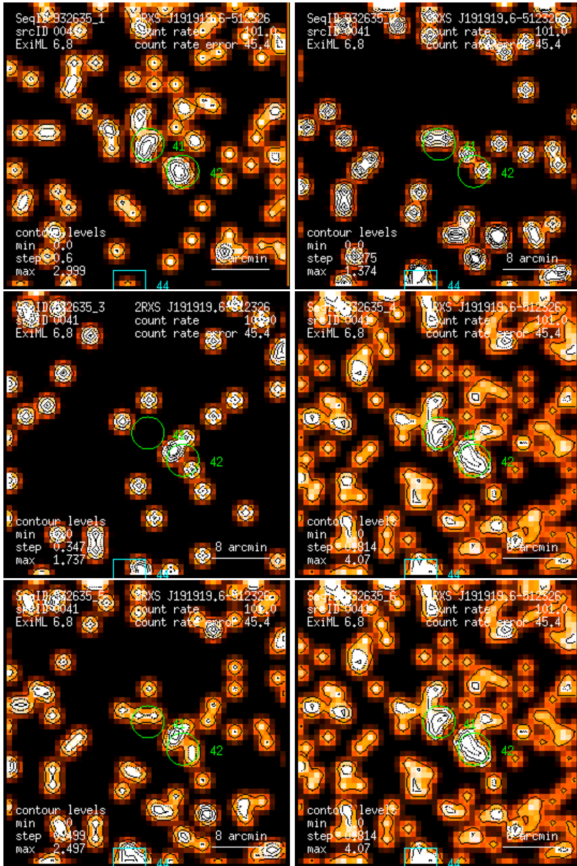
Figure 41: RASS 932635: detection 0041: band rate images, Gaussian filter: (1) PSPC channels 11 – 41, (2) 52 – 90, (3) 91 – 201, (4) 11 – 235, (5) 52 – 201, (6) 11 – 201. Broad band rates in counts/ks. Band rate contour levels in counts/ks/arcmin 2 .
