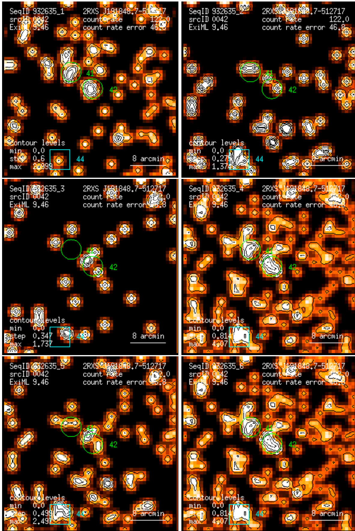
Figure 42: RASS 932635: detection 0042: band rate images, Gaussian filter: (1) PSPC channels 11 – 41, (2) 52 – 90, (3) 91 – 201, (4) 11 – 235, (5) 52 – 201, (6) 11 – 201. Broad band rates in counts/ks. Band rate contour levels in counts/ks/arcmin 2 .
