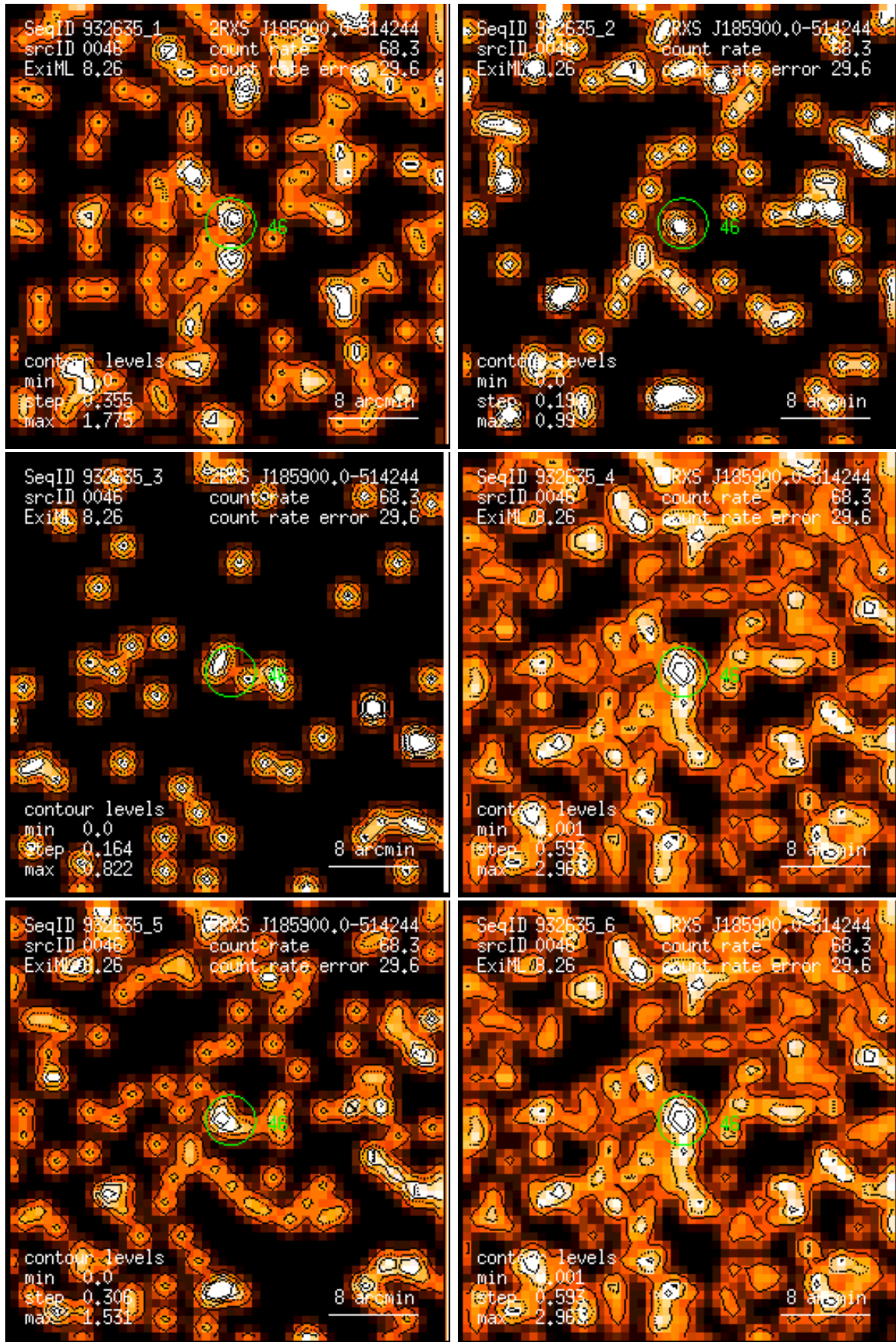
Figure 46: RASS 932635: detection 0046: band rate images, Gaussian filter: (1) PSPC channels 11 – 41, (2) 52 – 90, (3) 91 – 201, (4) 11 – 235, (5) 52 – 201, (6) 11 – 201. Broad band rates in counts/ks. Band rate contour levels in counts/ks/arcmin 2 .
